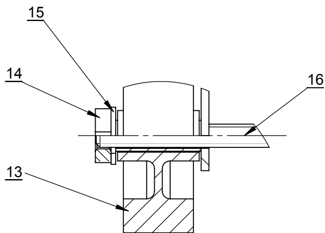
DETALL C (1 : 1)
