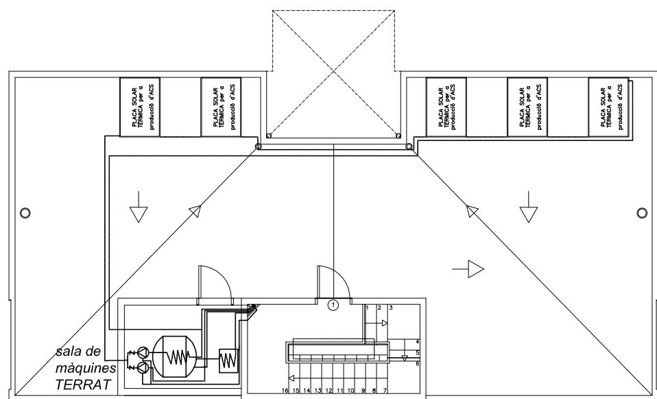
COBERTA TRANSITABLE
