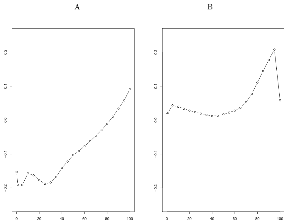
Figure 9: Japan, female, 1951-1990, right-singular vector components for: (A) Infectious Diseases; (B) Malignant Neoplasms.
