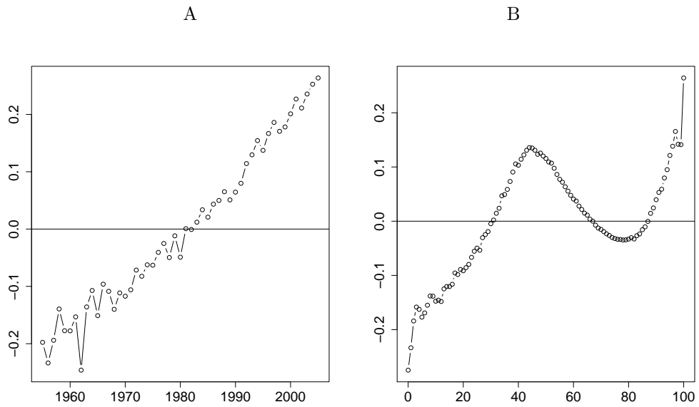
Figure 4: Hungary, male, 1955-2005: (A) Period Factor; (B) Age Factor.
