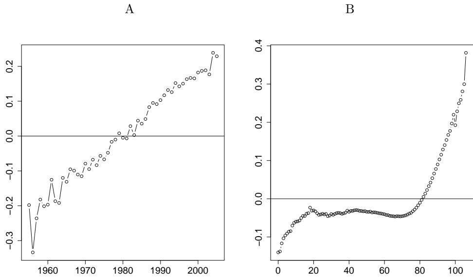
Figure 3: France, female, 1955-2005: (A) Period Factor; (B) Age Factor.
