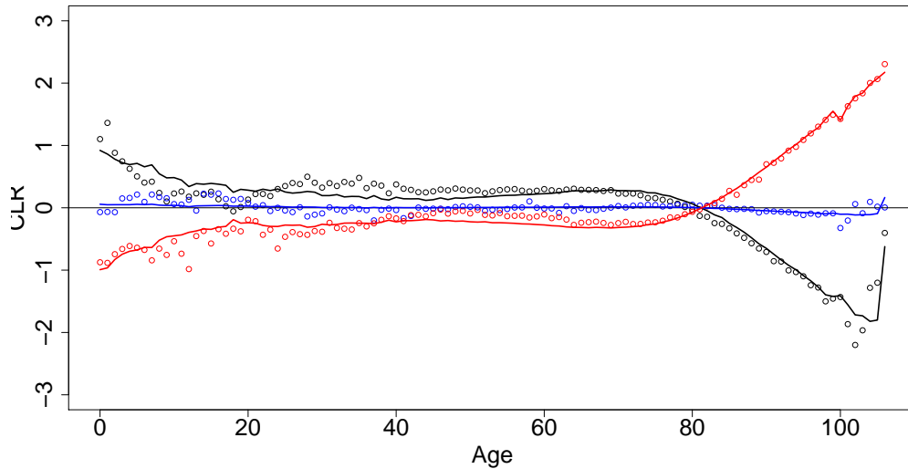
Figure 2: France, female, 1955-2005: CLR(centred d_x ) (points) and rank-2 model estimates (lines) for 1955 (black), 1979 (blue), 2005 (red).
