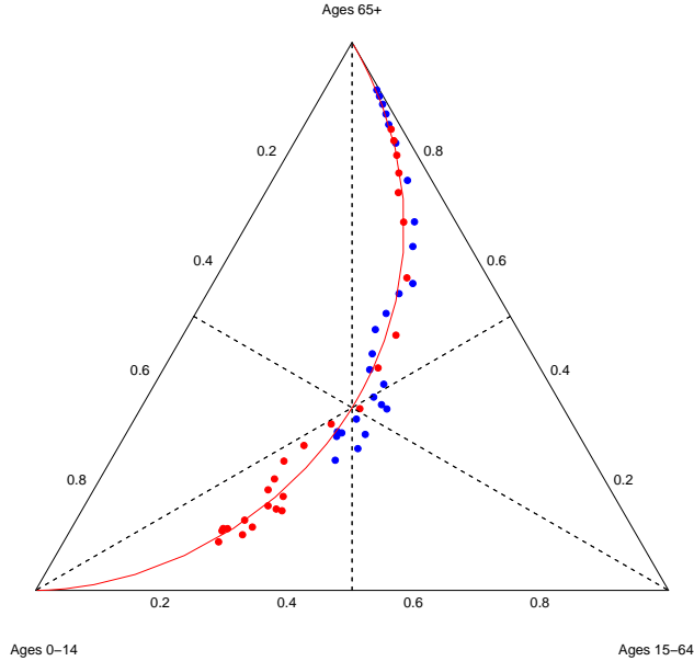
Figure 1: Compositional centring and the first Principal Component: original data (blue), centred data (red)
