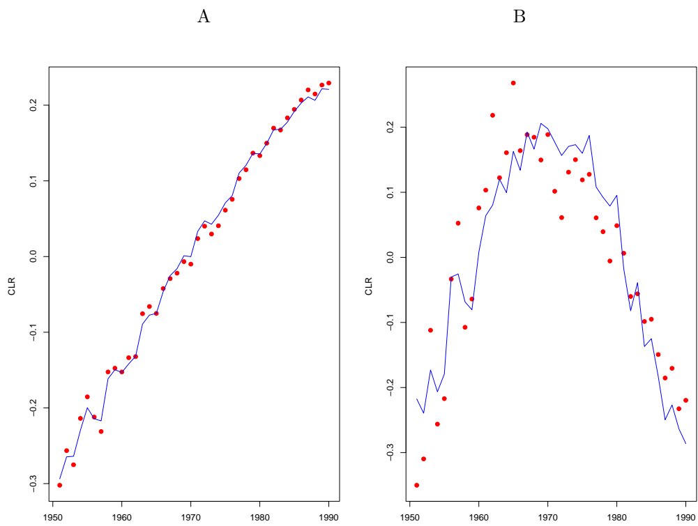
Figure 10: Japan, female, 1951-1990: (A) first left-singular vector; (B) second left-singular vector. Symbols: single decrement (red); multiple decrement (blue).
