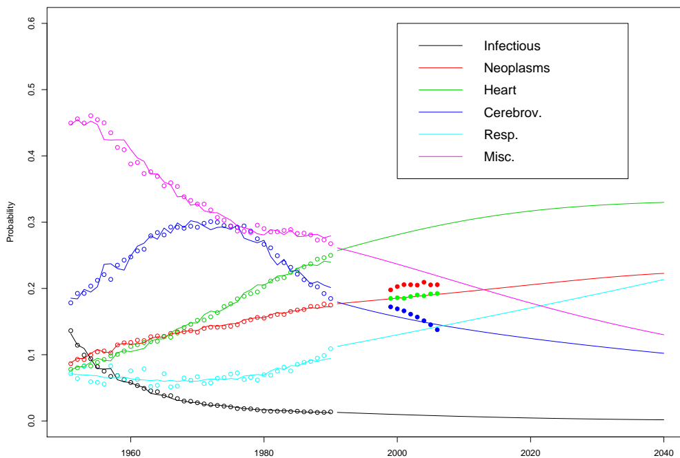
Figure 8: Japan, female period life-table probability at birth of dying from a specific cause: points = data, lines = estimates.
