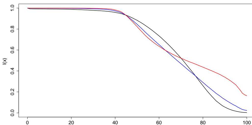
Figure 5: Hungary, male: survival probability ( \hat{l}_x ) in 2005 (black), 2050 (blue), 2100 (red).
