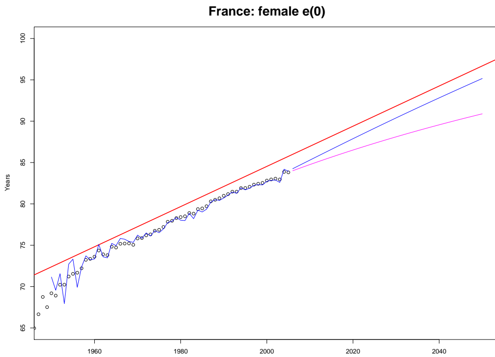
Figure 7: France, female: life expectancy at birth (circles), CoDa fitted and forecast (blue), Lee-Miller forecast (magenta), Best Practice (red).
