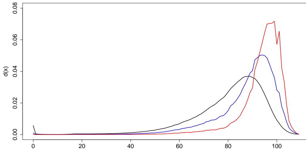
Figure 13: USA, female: \hat{d}_x in 2005 (black), 2050 (blue), 2100 (red).
