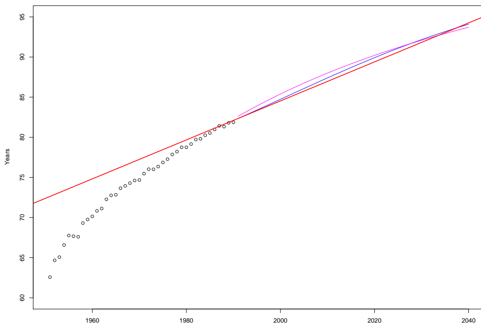
Figure 11: Japan, female, 1951-1990: life expectancy at birth (circles), single decrement forecast (magenta), multiple decrement forecast (blue), “best practice” (red).
