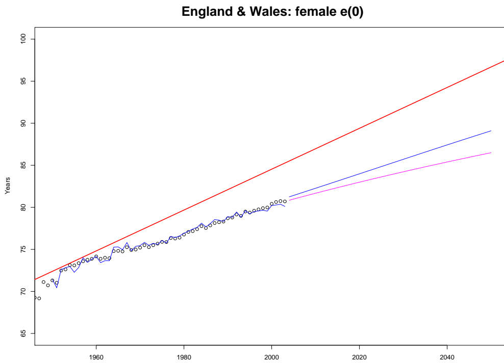
Figure 6: England and Wales, female: life expectancy at birth (circles), CoDa fitted and forecast (blue), Lee-Miller forecast (magenta), Best Practice (red).
