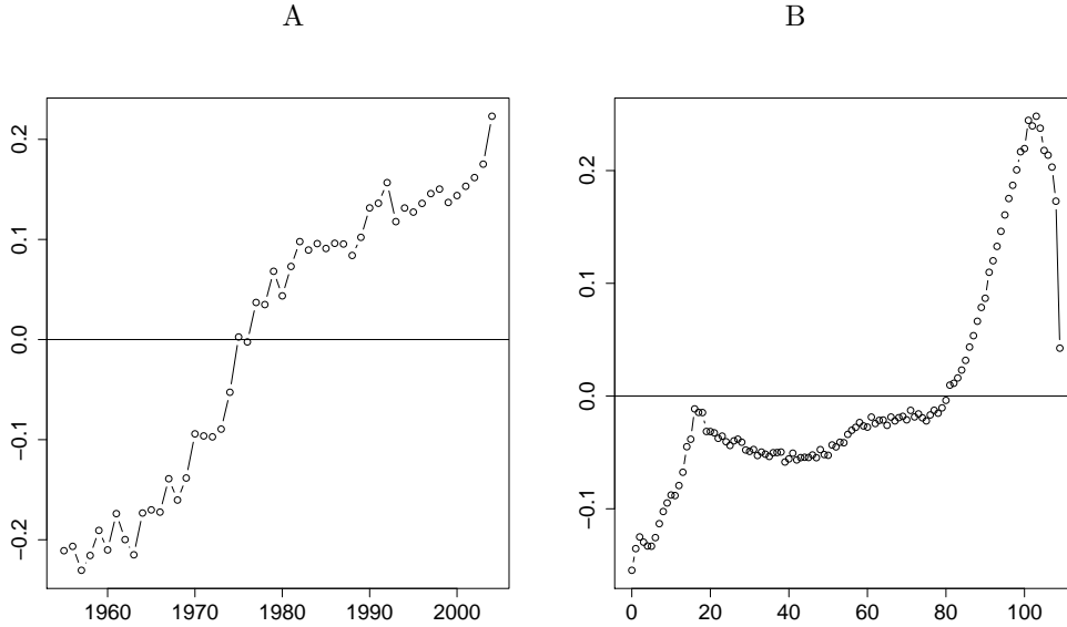
Figure 12: USA, female, 1955-2004: (A) Period Factor; (B) Age Factor.
