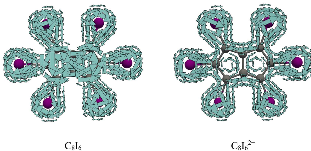
Fig. 7 Total current density maps plotted 1 Bohr above the molecular plane for C_8I_6 and C_8I_6^{2+} (a) and (b).
