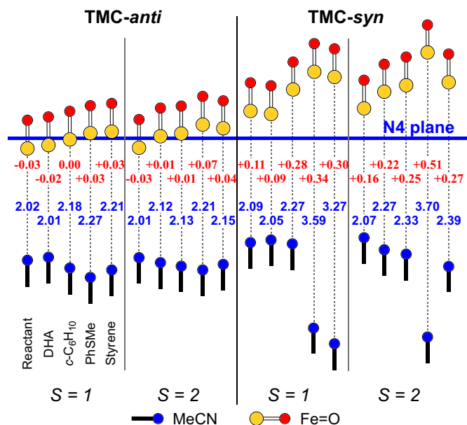
Fig. 2. Out-of-plane distances of the Fe=O and the CH 3 CN units relative to the N4 plane (B97-D3/TZ2P) for S = 1 and S = 2 states of TMC- anti and TMC- syn , for Fe=O reactants, and transition states of HAT (DHA, c-C 6 H 10 ) and OAT (PhSMe, styrene) substrates. Shown with dotted lines are the distances between iron and the axial CH 3 CN. Also indicated (in red, next to the Fe=O unit) are the Fe-oop distances.
