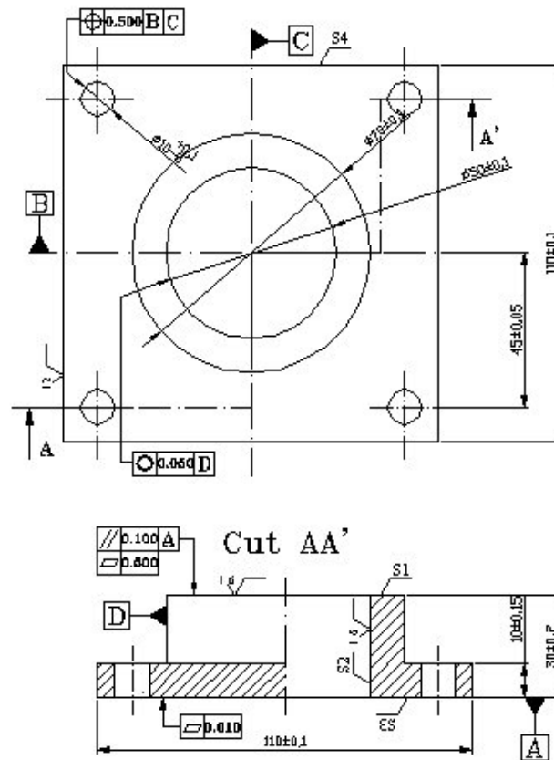
Figure 1: Example of a drawn part
