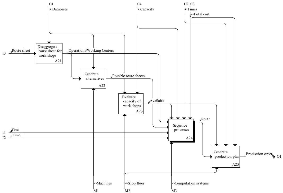
Figure 5: Production planning level in the IDEF model
