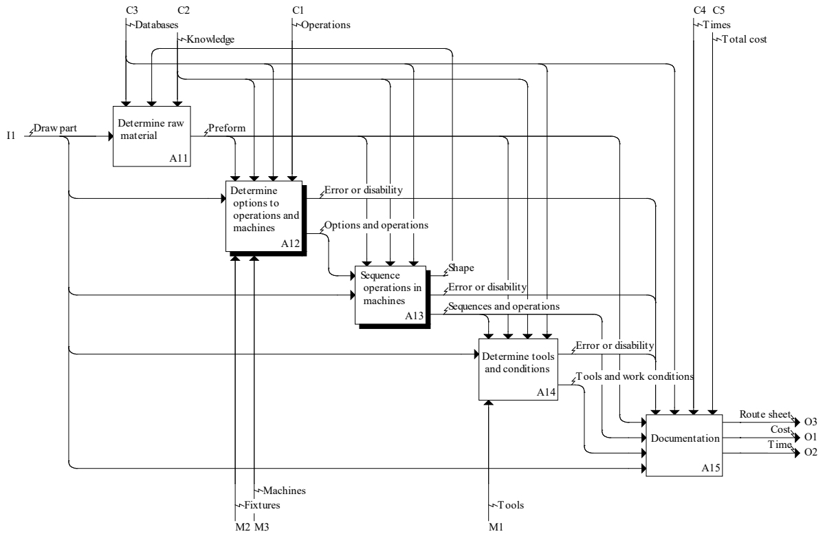
Figure 4: Process planning level in the IDEF model
