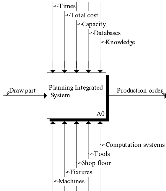
Figure 2: Initial level of the IDEF model
