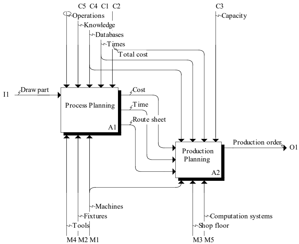
Figure 3: First level of the IDEF model
