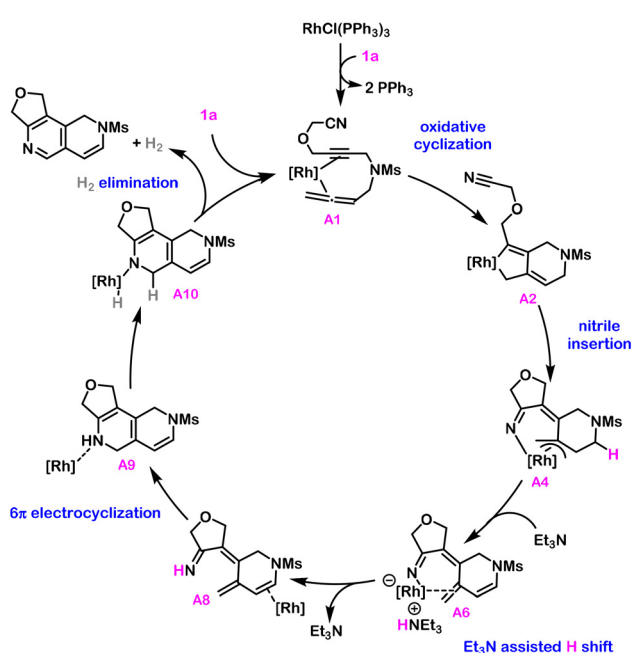
Scheme 3 Overall mechanism for the dehydrogenative [2 + 2 + 2] cycloaddition. [\text{Rh}] = \text{RhCl}(\text{PPh}_3)_3 .
