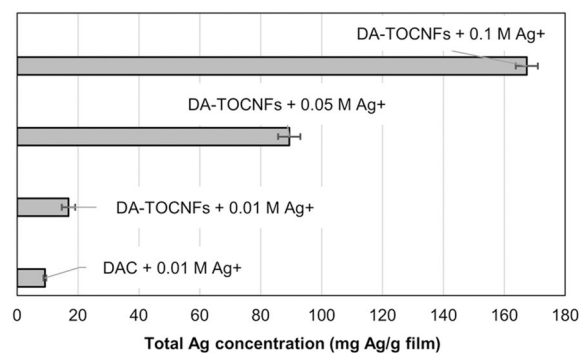
Fig. 6 Concentration of total silver, regardless of the oxidation degree, in oxycellulose/AgNP systems (on a dry weight basis), according to ICP-OES
