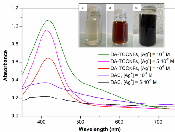
Fig. 1 Visible absorption spectra of the suspensions of DAC and DA-TOCNFs with AgNPs. The total solids content was 0.005 wt%, except for [\text{Ag}^+] = 5 \cdot 10^{-2} M and [\text{Ag}^+] = 10^{-1} M, for which it was 0.002 wt%. Inset image: photographs of DAC (a), DAC with AgNPs- 10^{-2} M (b), and DA-TOCNFs with AgNPs- 10^{-2} M (c). These suspensions had been freshly prepared at the time of the picture
