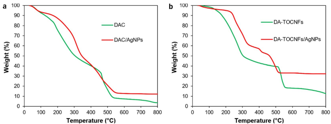
Fig. 8 Thermal degradation behavior of DAC, DAC/AgNPs (a), and DA-TOCNF, DA-TOCNFs/AgNPs, (b)
