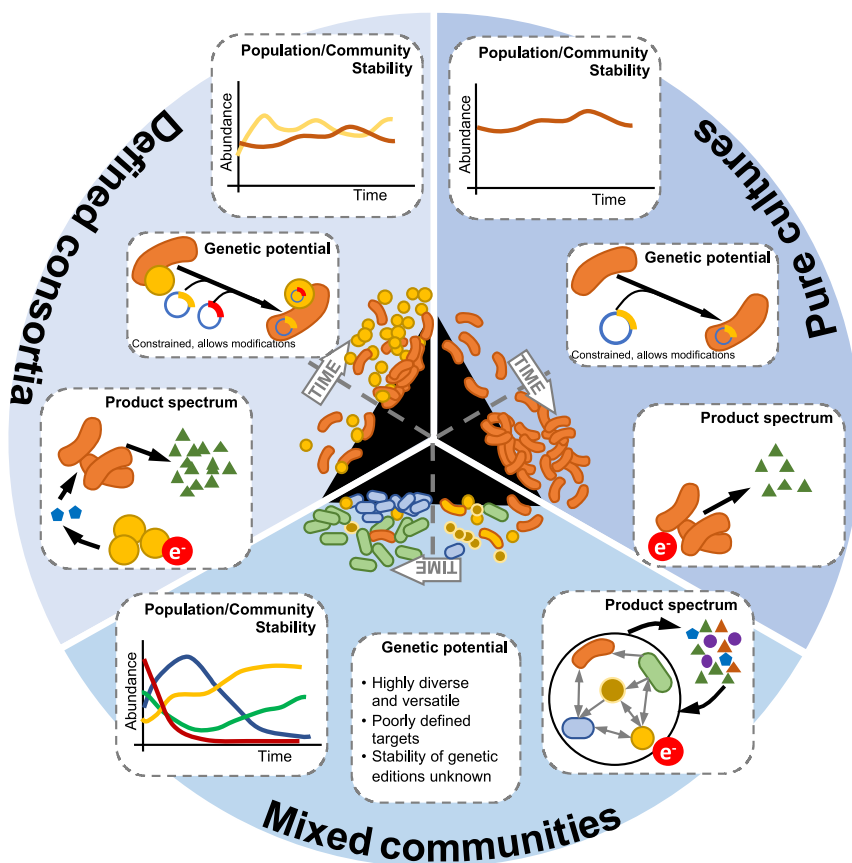
Fig. 1. Key properties of using pure microbial cultures, defined consortia, or mixed microbial communities (non-controlled composition) in MES reactors. Changes in size, morphologies and colours of cells depicted in the centre indicate different species (or taxa). The cathode surface is indicated as the black area in the centre of the figure. Cells may remain attached (direct contact) to the cathode or suspended in solution. White “TIME” arrows indicate example progressions of both cathode biofilm and suspended cells on an idealized MES reactor. Inserted graphs show some key features of Population community dynamics (depicted as growth kinetics), Genetic potential (briefly indicating editing possibilities), and ideal electron-to-product conversion and product spectrum (indicated here as small coloured dots). Pure cultures offer a limited product spectrum and conversion efficiency, but higher population stability (providing optimized conditions are applied). Gene edition of specific properties is possible. Defined consortia in co-cultures allow compartmentalization of the reactor (optimized reactions can be set for biofilm and bulk, independently) and may maximize energy-to-product conversion, increasing yields without a compromise of product selectivity. Gene editing of the consortium members is possible. Mixed bacterial populations are less predictable during start-up and operation and eventually evolve into unwanted activities if conditions are not maintained. Product spectrum increases due to larger metabolic potential and inter-species relationships. Some products can be used as substrates for bacteria thus minimizing yields. Genetic edition in these conditions is challenging due to the poor stability of engineered cells.
