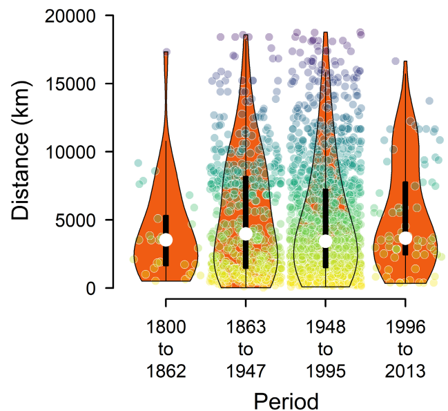
FIGURE 6 Violin plots of the distances between donor and recipient sites by period with homogeneous introduction rates and similar array of introduced species (see Methods and Figures S9 and S10 for information on how these periods were identified).
