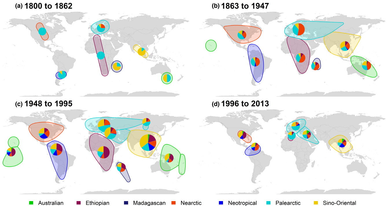
FIGURE 5 Introduction centres and origin of the introduced fish species for each period with homogeneous introduction rates and similar array of introduced species (see Methods and Figures S9 and S10 for information on how these periods were identified). The size of the pie charts is proportional to the log-transformed number of introduction events ( n_a=38 , n_b=649 , n_c=1836 and n_d=128 , introductions). Coloured areas encompass the coordinates of the locations clustered in each centre and pie chart. An analogous figure depicting the most frequently introduced species in each period can be found in Supplementary material S1 (Figure S11).
