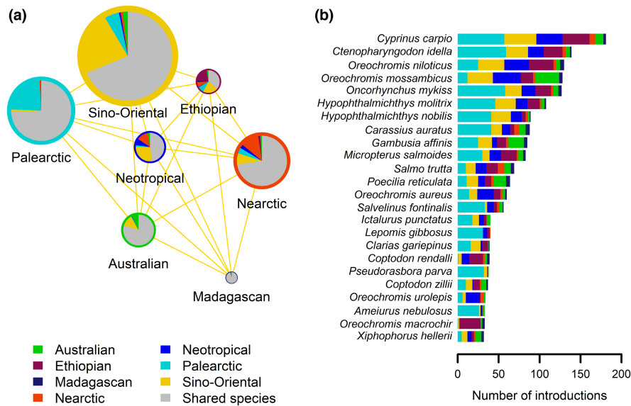
FIGURE 3 (a) Undirected graph based on the Bray–Curtis dissimilarity between the total number of introductions per species and biogeographic region. Edge length is proportional to the inverse distance between regions (1–Bray–Curtis dissimilarity). Pie charts depict the per cent of shared species (grey) and exclusive species (i.e., introduced in one single biogeographic region). The origin of the exclusive species has been split by biogeographic region of origin. Pie chart sizes are proportional to the total number of introduction events. (b) Barplot of the 24 most frequently introduced species (41.9% of all known introduction events) by recipient biogeographic region.
