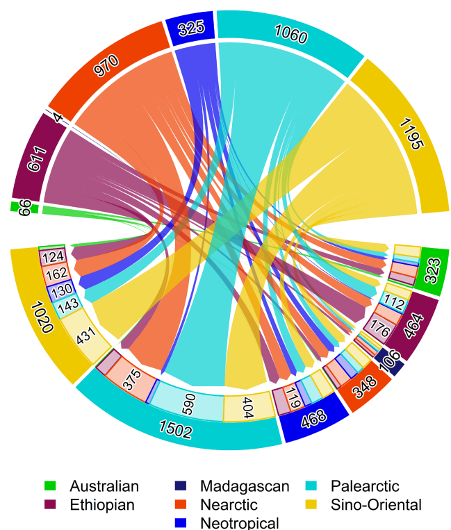
FIGURE 2 Flow diagrams of the total number of freshwater fish introduction events ( n=4233 ). The numbers indicate the total number of events, including repeated introductions. An analogous figure for the number of species introduced can be found in Supplementary material S1 (Figure S6).
