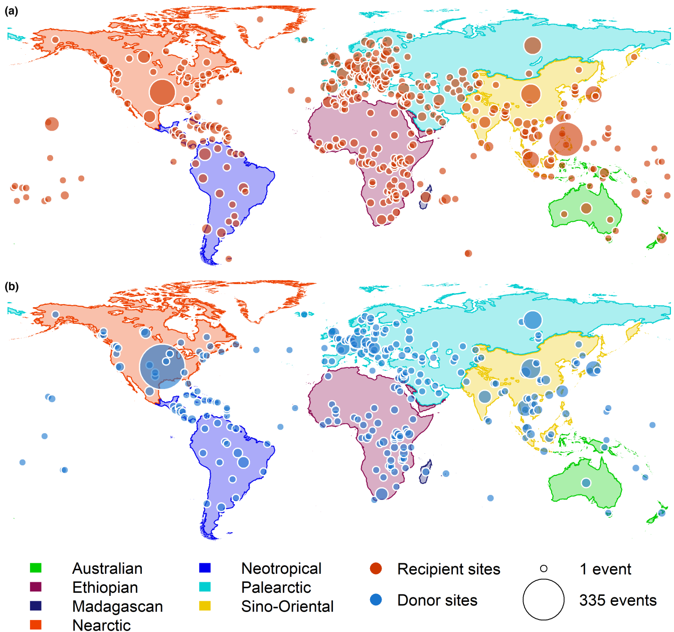
FIGURE 1 Biogeographic regions and recipient (a) and donor (b) locations available in the FishBase dataset (coordinates of the locations were obtained at the highest available resolution: country, basin, river/lake or site). The sizes of the circles are proportional to the number of introductions in each location. A figure connecting donor and recipient sites can be found in Supplementary material S1 (Figure S2).
