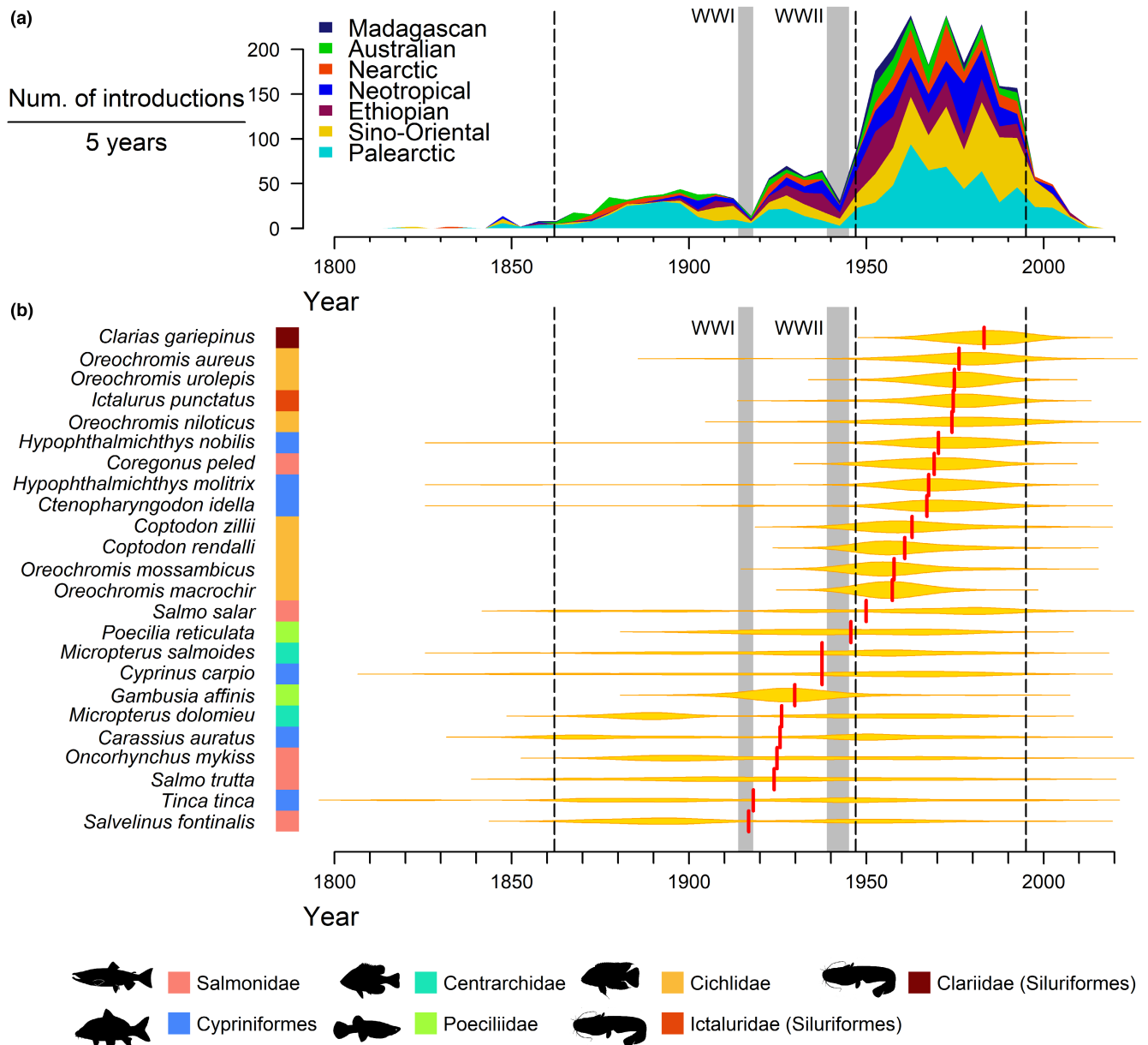
FIGURE 4 (a) Number of introductions per five-year period and biogeographic region. The reported introductions markedly diminished during World War I (WWI) and World War II (WWII) (grey strips). Dashed grey lines indicate the breakpoints of the four distinct introduction periods with homogeneous introduction rates and introduced species (see Methods and Figures S8 and S9 for information on how these periods were identified). (b) Violin plots of the introduction dates of most introduced species with known introduction dates. The red segments depict the mean values. Grey strips indicate WWI and WWII and dashed grey lines the breakpoints of the four distinct introduction periods.
