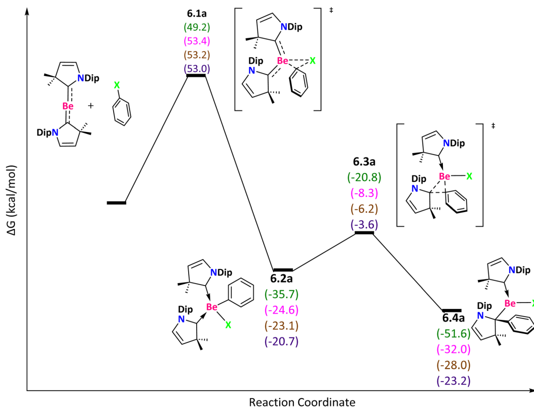
Fig. 7 Reaction mechanism determined at the \omega\text{B97X-D}/\text{def2-TZVP}(\text{SMD}:\text{toluene})//\omega\text{B97X-D}/\text{def2-SVPP} level. X = F (green), Cl (pink), Br (brown), and I (purple).
