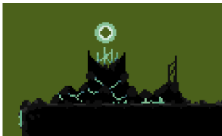
Figura 10.8.1: Checkpoint desactivat
