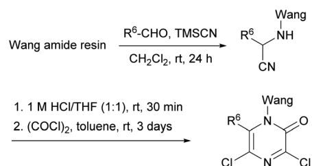
Scheme 14 Solid-phase synthesis of 3,5-dichloro-2(1H)-pyrazinones.
