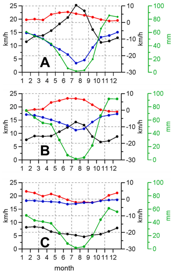
Fig. 6. Monthly time series of the wind intensity, west-east (Ux) and south-north (Uy) components of the wind, and precipitation rates (P) in the Portuguese Coast (POR) (A), Gulf of Cádiz (GC) (B), and Alboran Coast (Alb) (C). Wind intensity in km/h (black lines and left y-axis); west-east component in km/h (Ux, red lines and right y-axis); south-north component in km/h (Uy, blue lines and right y-axis); precipitation rates in mm (green lines and green y-axis).
