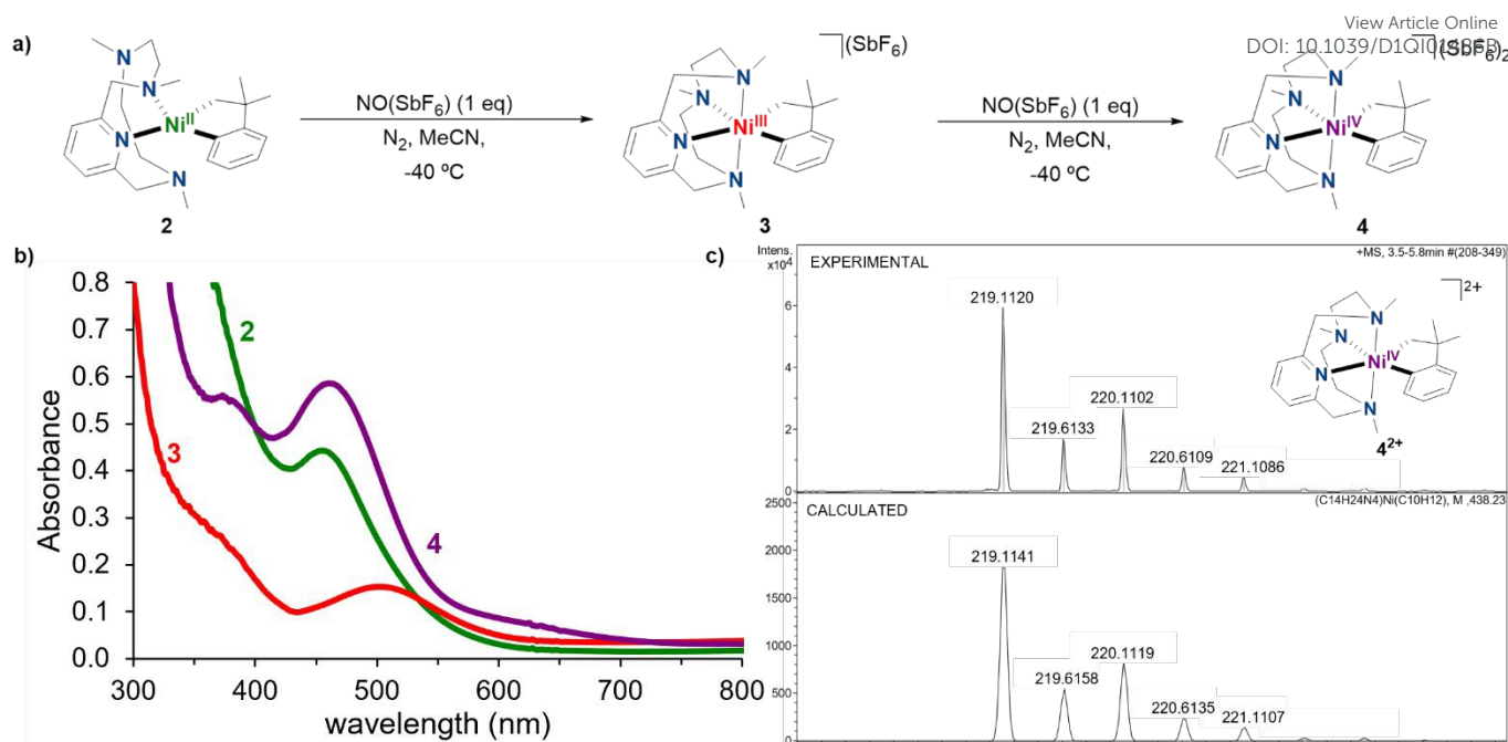
Fig. 5 a) Step-wise one-electron oxidation to nickel(IV) from 2 using \text{NO}(\text{SbF}_6) as oxidant; b) UV-vis characterization of complexes 2 , 3 and 4 obtained by consecutive one-electron oxidation of 2 with \text{NO}(\text{SbF}_6) , respectively, and c) Cryo-HR-MS of 4 showing the dicationic peak ( 4^{2+} ) at m/z = 219.1120 (top) and simulation of its isotopic pattern (bottom).
