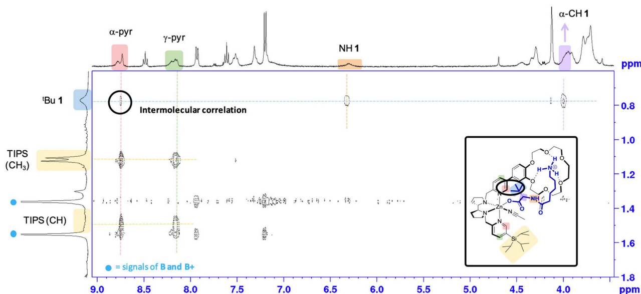
Figure 4. Intermolecular NOESY correlation between deprotonated 1 and ^{CR,TIPS}Mn , indicating carboxylate coordination (proximity between the ^tBu group of 1 and the pyridine \alpha -C-H signals of the complex).
