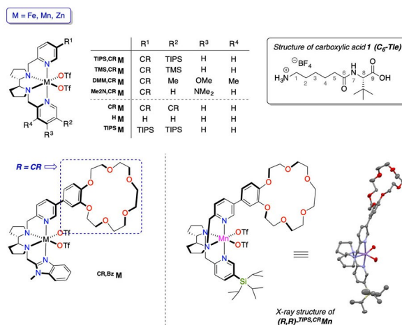
Figure 2. Structure of catalysts used in this work and carboxylic acid 1 . On the bottom right the crystal structure of (R,R)- CR TIPS 2 CR Mn (50 % probability ellipsoids) is displayed. Triflate groups, except for O atoms directly bound to the metal, are omitted for clarity. [CR = 18-benzo-crown-6-ether].
