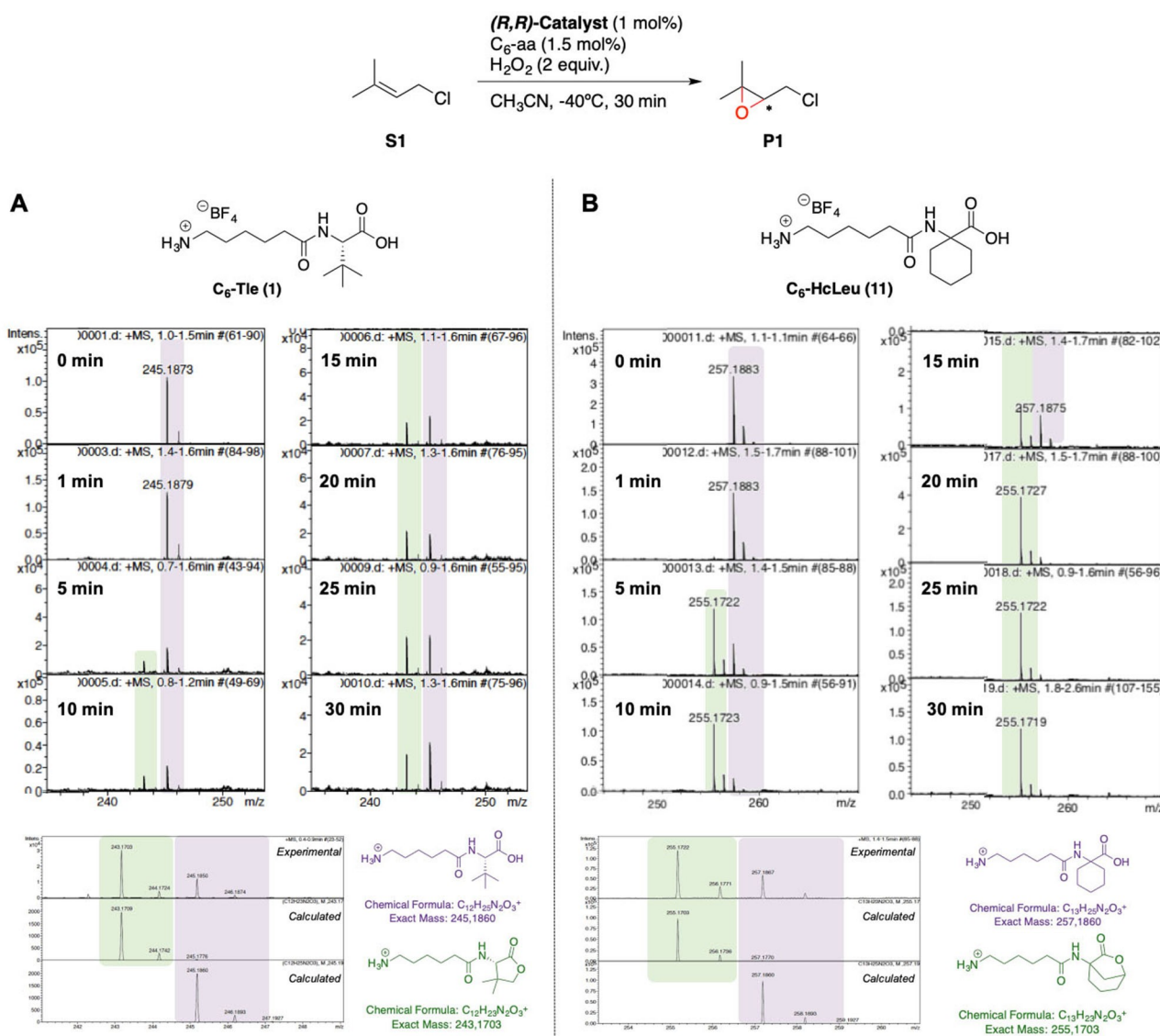
Figure 7. HRMS time-course analysis of the epoxidation of S1 using (R,R) - CR,TIPS Mn/1 (A) and (R,R) - CR,TIPS Mn/11 (B).
