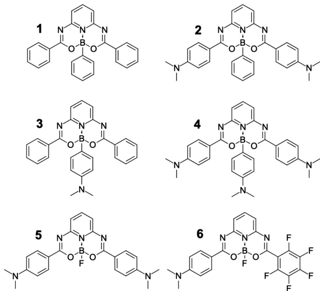
Fig. 3 The studied compounds 1–6.
