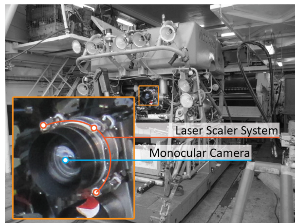
Fig. 16. ROV VICTOR 6000 (IFREMER) with enlarged camera and laser scaler system.
