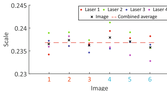
Fig. 19. Estimated scale factors for FPA model, per laser and per image, using our fully unconstrained method. Colour of image numbers (x axis) corresponds to locations shown in Fig. 18. (For interpretation of the references to colour in this figure legend, the reader is referred to the web version of this article.)
