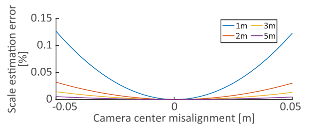
Fig. 7. Error in the estimation of scale using partially constrained method due to the misalignment of camera center with the laser pair.
