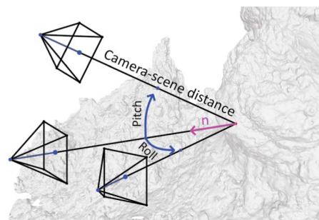
Fig. 10. Definition of perspective angles and camera-scene distance used in the generation of the evaluation data.
