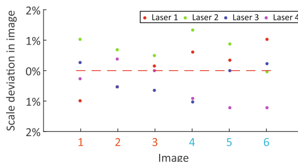
Fig. 20. Deviation of estimated FPA model’s scales, using our fully unconstrained method FUM, and for each laser in each image.
