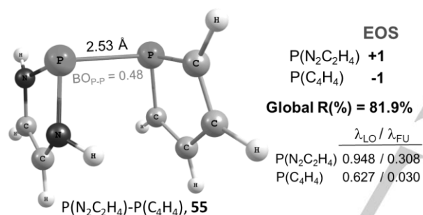
Figure 5. N-heterocyclic phosphonium-phospholide anion adduct ( 55 ) and results of the EOS analysis. P-P distance (Å) and bond order are also indicated.
