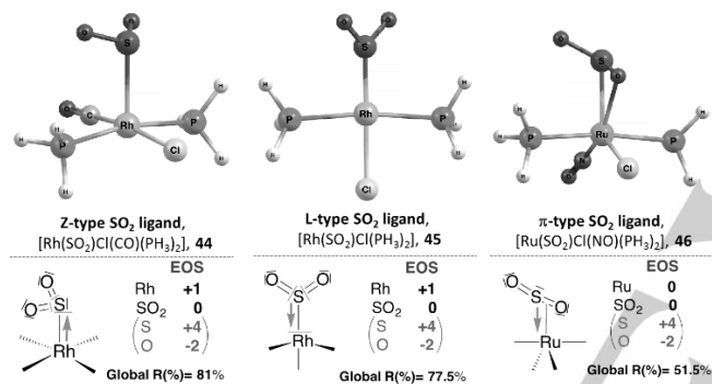
Figure 3. Binding modes of SO 2 ligand and results of EOS analysis (see text).
