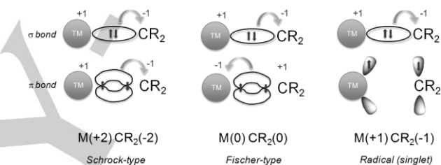
Figure 6. Pictorial representation of singlet Schrock, Fischer and radical TM-carbene complexes and the expected OS.
