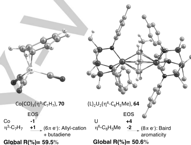
Figure 4. Sample cases of \pi -system ionicity driven by Baird's aromaticity (right) and conjugated segments left), and results of the EOS analysis.
