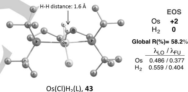
Figure 2. Representation of \text{Os}(\text{Cl})\text{H}_2(\text{L}) complex ( 43 ) (hydrogen atoms in the ligands omitted for clarity) and results of the EOS analysis.
