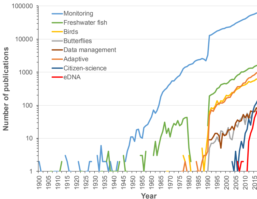
Figure S1.1. Historical variation in the number of publications on monitoring and related topics according to a literature search in the Web of Science. The search was performed on 27 February 2018 (but excludes papers published in 2018) using “Science Citation Index Expanded” (topics: monitoring” and freshwater fish*” or “bird*” or “butterfl*” or data management” or “adaptive” or “citizen-science” or “environmental DNA”). Notice the logarithmic scale in the number of publications and that the Web of Science started to systematically include the abstracts of papers in 1990, hence producing a general increase that year.
