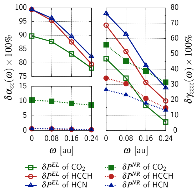
Fig. 1 Relative changes of electronic ( P^{\text{EL}} ) and vibrational ( P^{\text{NR}} ) contributions to longitudinal polarizabilities (left panel) and second hyperpolarizabilities (right panel) upon applied confining potential. \delta P^{\text{X}}(\omega) = P^{\text{X}}(\omega)/(P^{\text{EL}}(0) + P^{\text{NR}}(0)) .
