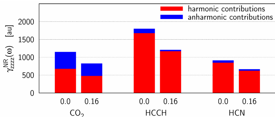
Fig. 2 Breakdown of the longitudinal nuclear relaxation second hyperpolarizability into harmonic and anharmonic contributions upon applied confining potential ( \omega ).
