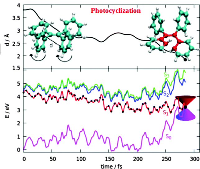
Figure 6. Interannular CC distance (upper panel) and electronic state potential energies (lower panel, S 0 /S 1 /S 2 /S 3 shown in magenta/red/blue/green) as a function of time for a representative trajectory undergoing photocyclization. The actual (running) electronic state is shown in black. All the energies are relative to the initial (0 fs) energy. Initial (0 fs) and final (close to the CI) molecular structures are shown. Trajectories computed at the PBE0/def2-SVP level. Adapted from Ref. [53] with permission from the PCCP Owner Societies.
