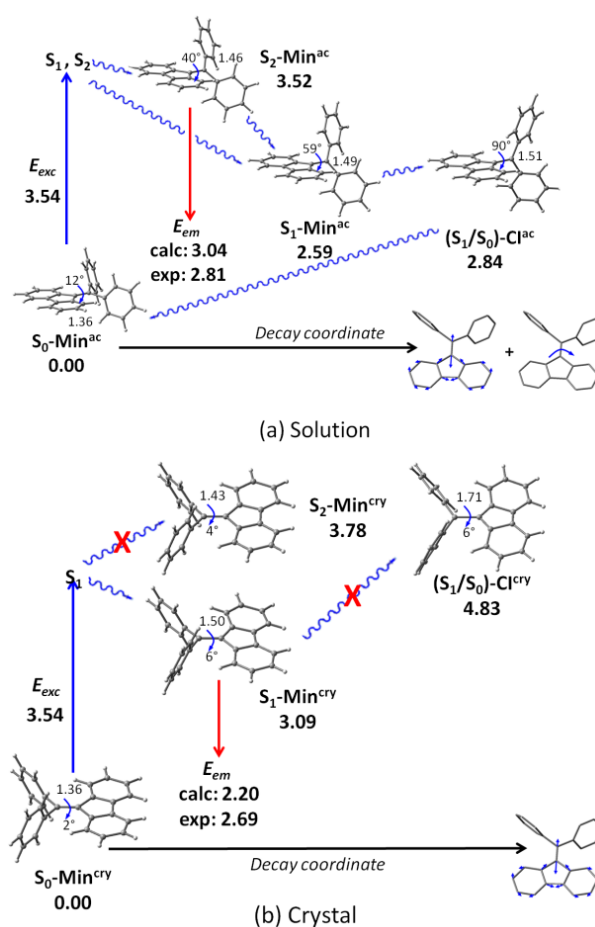
Figure 3. Calculated mechanisms for the photophysics of DPDBF (a) in acetonitrile and (b) in the solid phase (crystal). Structural parameters: C-C distance of the exocyclic double bond and bond torsion angle. Straight blue and red arrows: excitation and emission. Curled blue arrow: vibrational relaxation and internal conversion. Energies in eV. Adapted from Ref. [43] with permission from The Royal Society of Chemistry.
