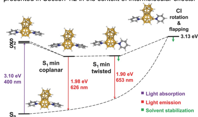
Figure 13. Scheme of B_{18}H_{20}(NC_5H_5)_2 photophysics based on CASPT2//CASSCF computations. Reprinted from Ref. [48] with permission from John Wiley and Sons.
