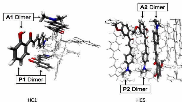
Figure 16. Arrangements of dimers in molecular crystals of HC1 and HC5. Adapted with permission from Ref. [92]. Copyright 2017 American Chemical Society.
