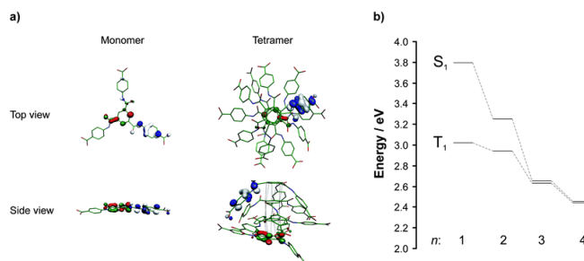
Figure 18. HOMO (blue/white) and LUMO (red/green) orbitals for the monomer and tetramers of BTA. Energies of singlet and triplet excited state with the number of molecules in the aggregates. Reproduced from Ref. [96] with permission from the Royal Society of Chemistry.
