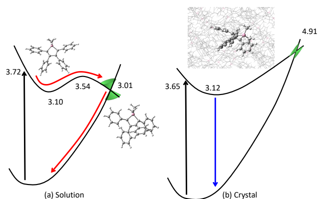
Figure 9. Summary of the proposed decay paths of DMTPS (a) in solution and (b) in the crystal. Adapted from Ref. [38] with permission from the Royal Society of Chemistry.
