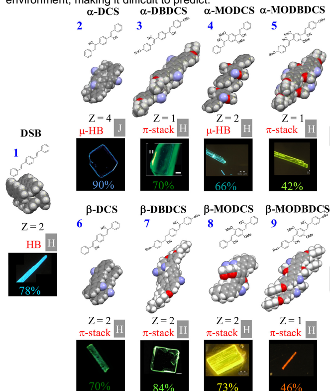
Figure 15. Quantum efficiencies and features of the crystal structures for series \alpha and \beta of DSB derivatives investigated in Ref. [1]. Relevant features of the crystal structure including dominant arrangements (HB: herringbone and \pi -stack) and the dominant couplings are specified (H vs J couplings). Adapted with permission from Ref [1]. Copyright 2017 American Chemical Society.
