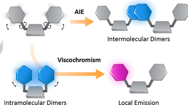
Figure 19. Scheme of the two processes proposed to explain luminescence in phenyl-ring molecular rotors. Reproduced with permission from Ref. [98]. Copyright 2017 American Chemical Society.
