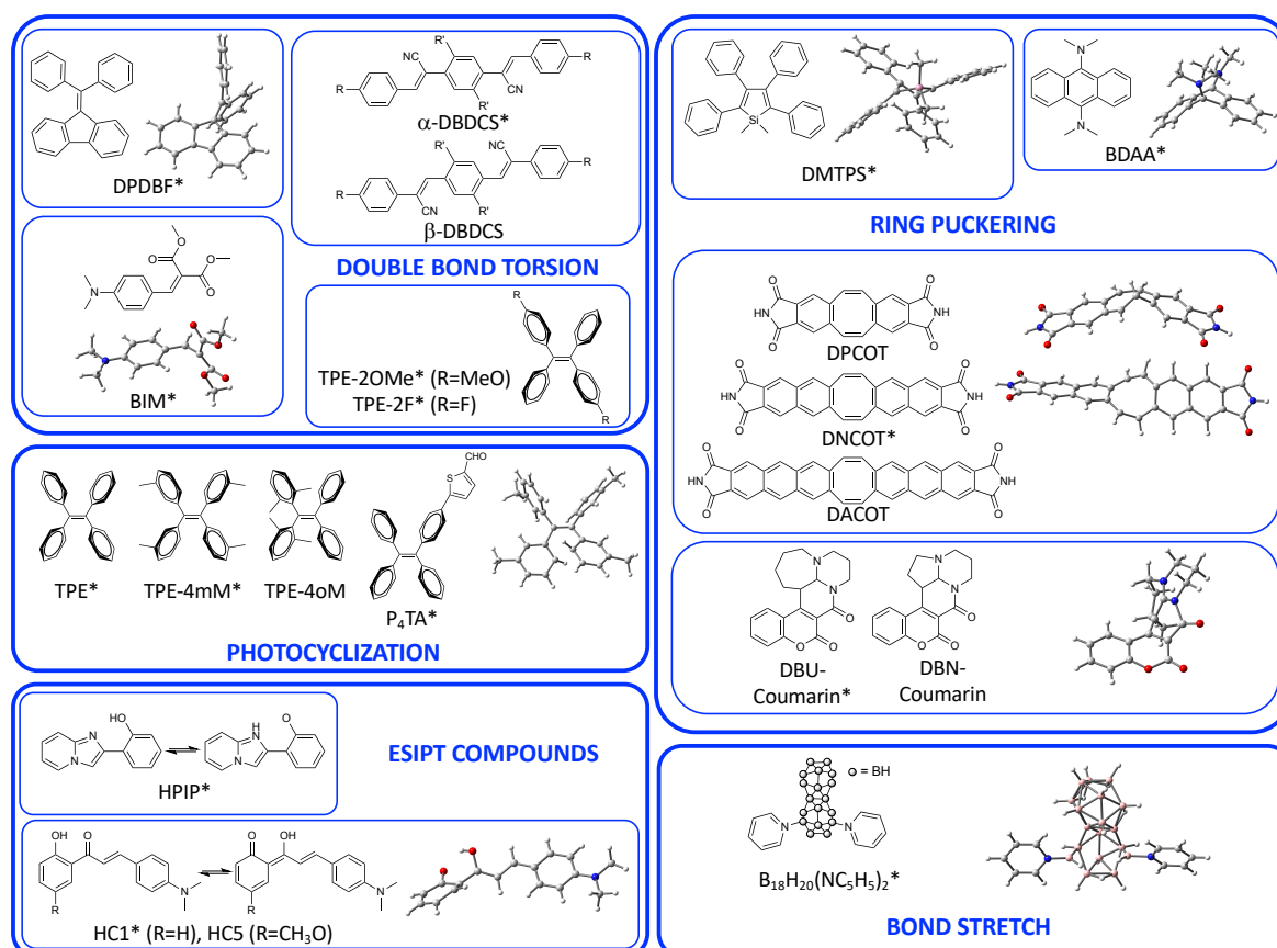
Figure 2. Overview of molecules discussed in Section 3. AIEgens following the RACI model are labelled with an asterisk. The molecular models correspond to the CI structures responsible for radiationless decay in solution.
