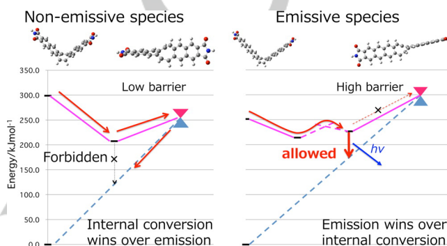
Figure 10. Schematic representation of the mechanisms governing AIE in DNCOT (left panel) and emission in solution in DACOT (right panel). Reproduced with permission from Ref. [46], https://pubs.acs.org/doi/10.1021/acs.jpca.5b07682 . Copyright 2015 American Chemical Society (ACS). Further permissions related to this material should be related to the ACS.
