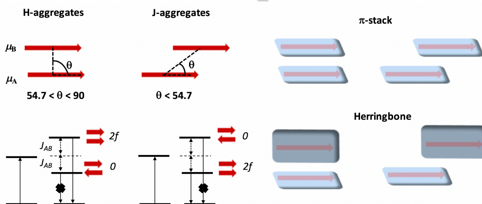
Figure 14. Illustration of the orientation of transition dipole moments ( \mu ) for J- and H-aggregates. For the H-aggregates emission is forbidden (oscillator strength, f = 0 ), while for J-aggregates the transition dipole moment is twice the value of the molecule ( 2f ). On the right, \pi -stack and herringbone configurations in dimers of planar aromatic molecules are illustrated.
