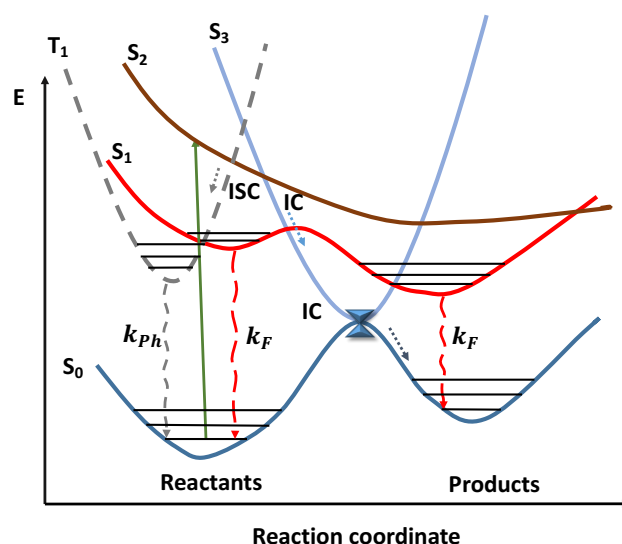
Figure 1. Radiative ( r ) and non-radiative ( nr ) processes in a typical PES. Only few vibrational states are shown for illustrative purposes.
