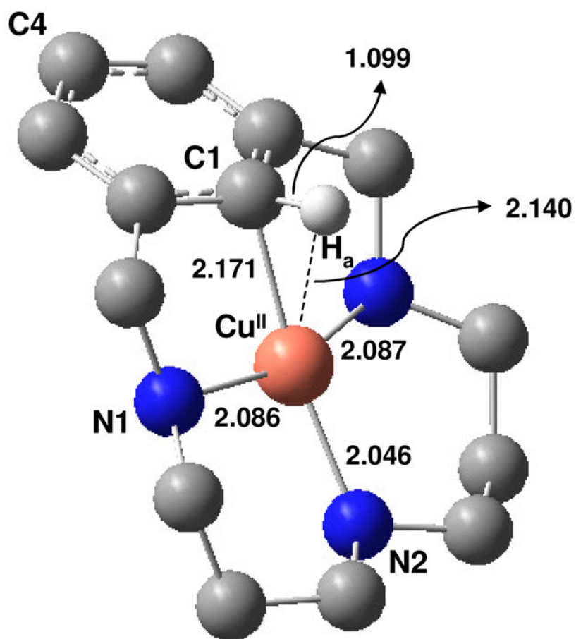
Figure 2. DFT optimized model of 1 with selected bond distances (Å). All hydrogen atoms are excluded except for the \text{H}_a involved in the \text{C-H}_a \cdots \text{Cu}^{\text{II}} interaction.
