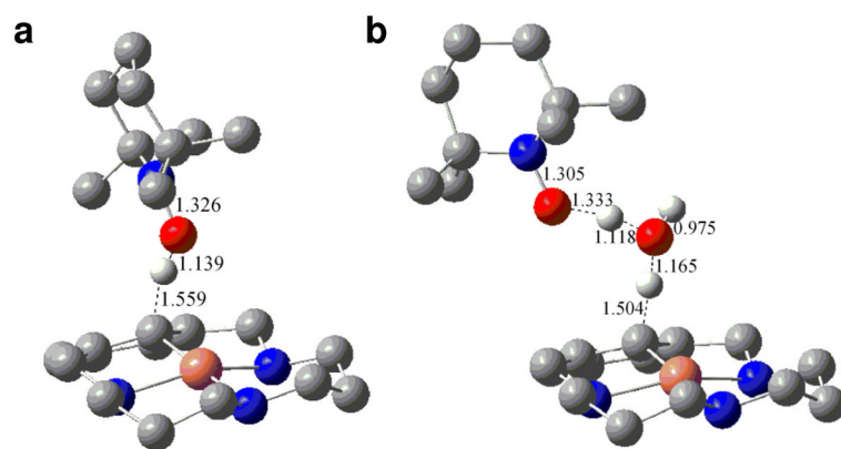
Figure 5. DFT optimization of transition states for (a) the bimolecular reaction between complex 1 and TEMPO with an energy barrier of 22.9 \text{ kcal mol}^{-1} , and (b) the same reaction assisted by an intervening water molecule with an energy barrier of 9.0 \text{ kcal mol}^{-1} .
