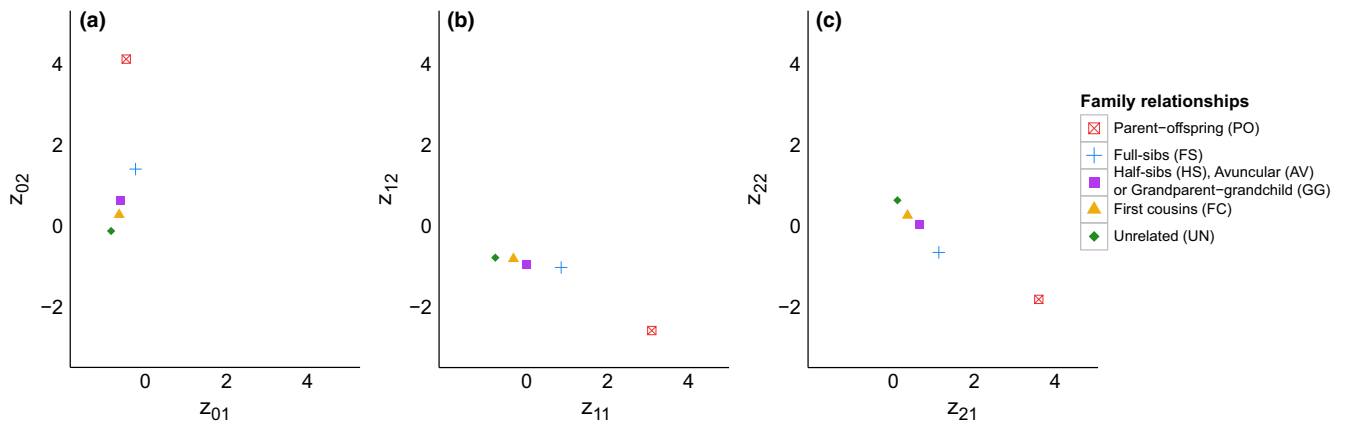
FIGURE 4 IIR-coordinates of the IBS proportions for five pairs of individuals from the Maya population. a. z_0 = (z_{01}, z_{02}) . b. z_1 = (z_{11}, z_{12}) . c. z_2 = (z_{21}, z_{22})
