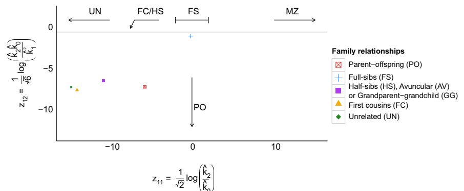
FIGURE 6 Ilr-coordinates \mathbf{z}_1 = (z_{11}, z_{12}) of the estimated Catterman coefficients (\hat{k}_0, \hat{k}_1, \hat{k}_2) for five pairs of individuals from the Maya population
