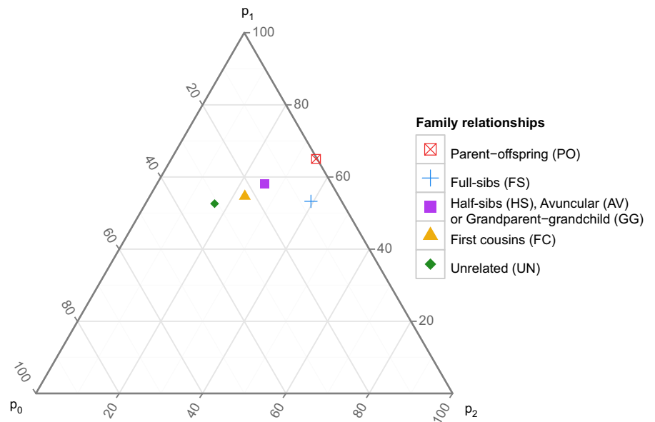
FIGURE 3 Ternary diagram of the IBS proportions for five pairs from the Maya population
