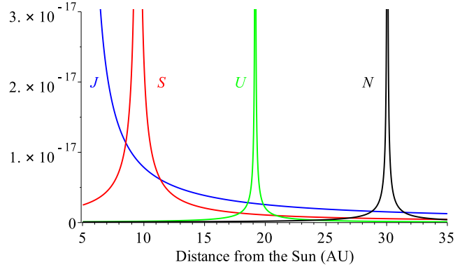
Figure 2. Values of the gravity potential (in \text{au}^2 \text{s}^{-2} ) of the Earth (E), Mars (M) and Jupiter (J) in the heliocentric region including the orbits of the Earth and Mars (left), and gravity potential of Jupiter (J), Saturn (S), Uranus (U) and Neptune (N) in the heliocentric region corresponding to the outer Solar system.
