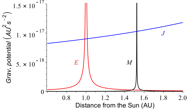
Figure 2. Values of the gravity potential (in \text{au}^2 \text{s}^{-2} ) of the Earth (E), Mars (M) and Jupiter (J) in the heliocentric region including the orbits of the Earth and Mars (left), and gravity potential of Jupiter (J), Saturn (S), Uranus (U) and Neptune (N) in the heliocentric region corresponding to the outer Solar system.
