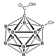
1- \text{CH}_3 -2- \text{COOH} -1,2- closo - \text{C}_2\text{B}_{10}\text{H}_{10} ( LH )
