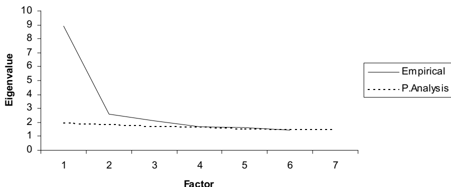
FIGURE 1. Scree plot and parallel analysis for factor analysis.
