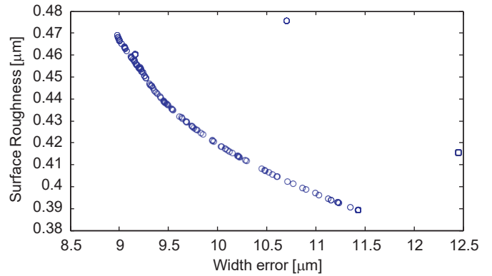
Fig. 10. Pareto frontier of optimal surface roughness and width error of laser milling parameters.
