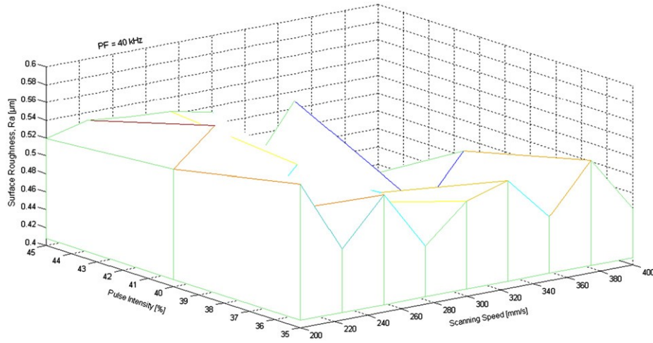
Fig. 6. Effect of scanning speed and pulse intensity on surface roughness (PF ¼ 40 kHz).
