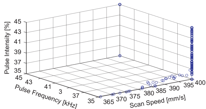
Fig. 13. Decision variable space for optimal laser milling parameters for depth and width.
