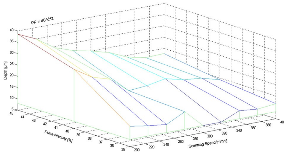
Fig. 4. Effect of pulse intensity and scanning speed on micro-channel depth (PF = 40 kHz).
