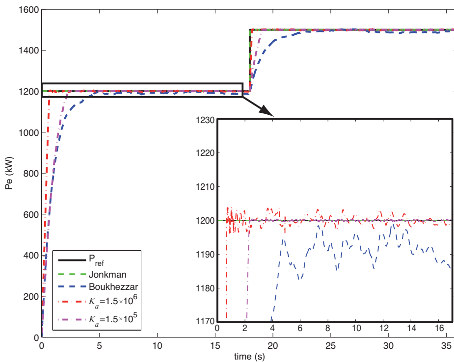
Figure 5. Power output.
