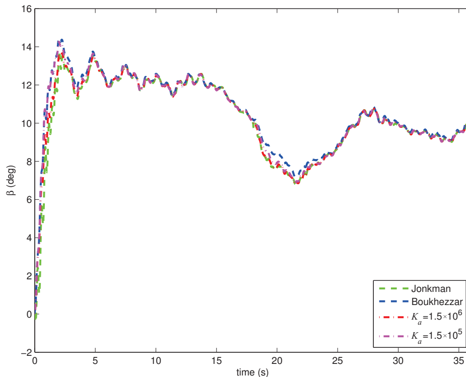
Figure 6. Pitch control.
