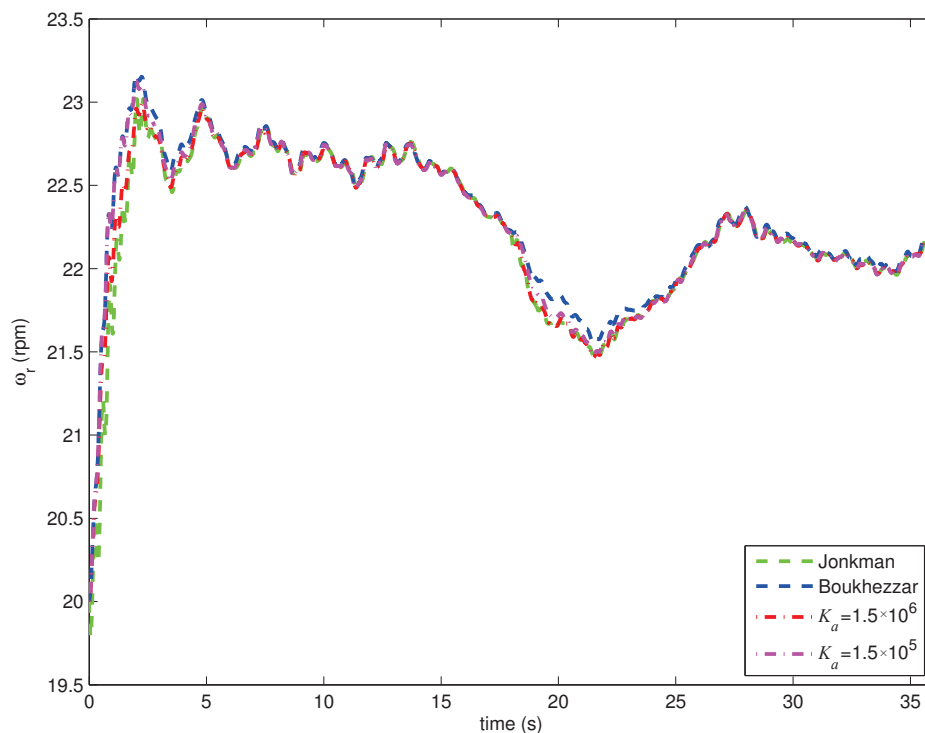
Figure 4. Rotor speed.
