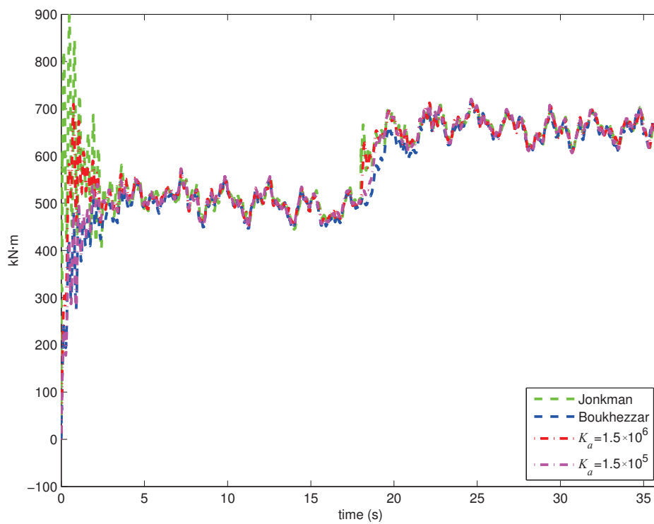
Figure 10. Tower top/yaw bearing roll moment.
