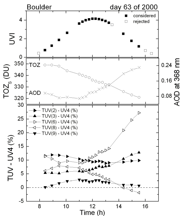
Fig. 10. Upper panel: Measured UVI on day 63 in Boulder as a function of time. Open squares were rejected from the study due to lack of AOD measurements for those times. Center panel: Concurrent TOZ_S and AOD as a function of time. Lower panel: relative differences between UVI model and measurement for modelling cases TUV(2,3,6,8,9) as a function of time.
