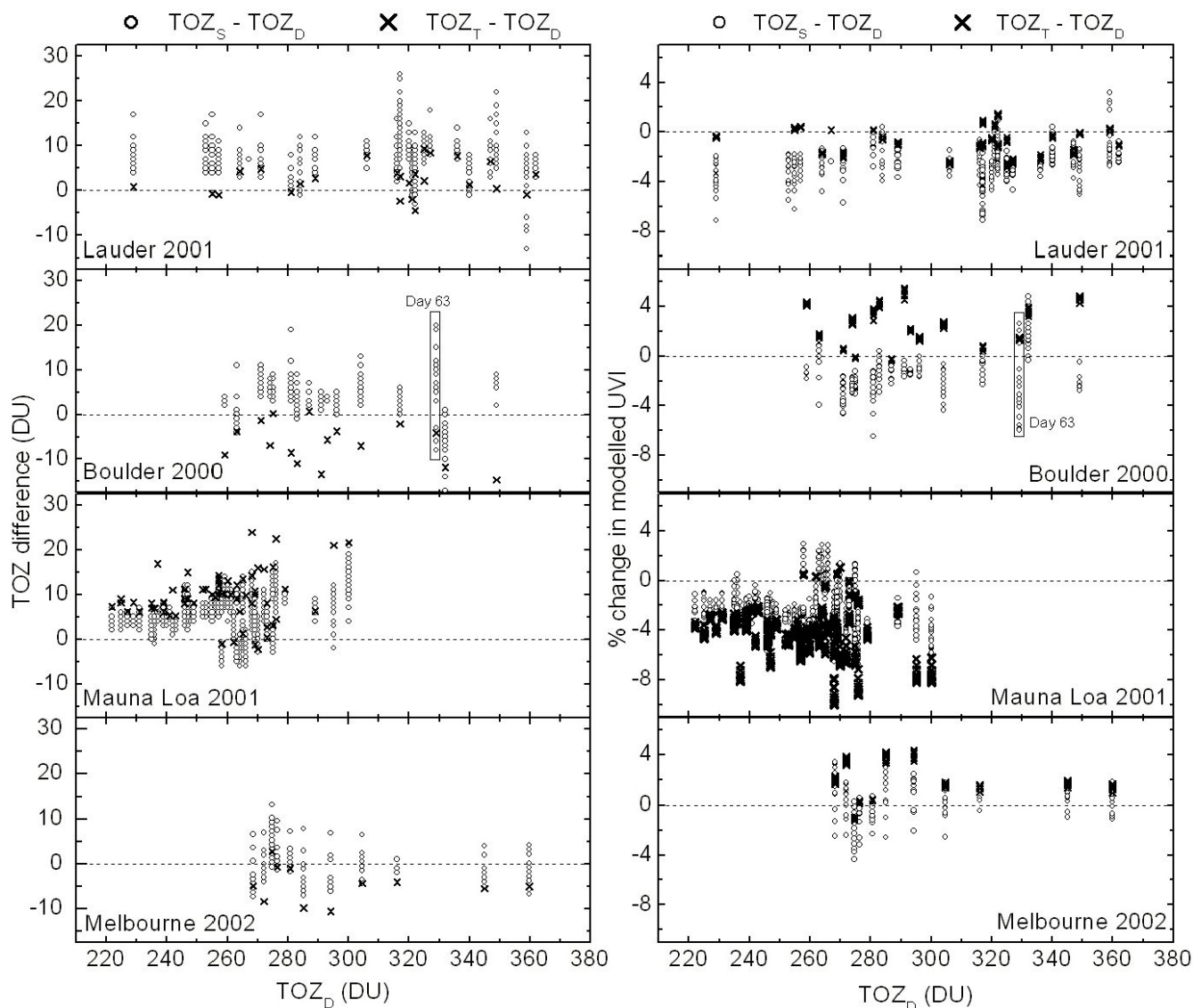
Fig. 2. Left panel: Differences in ozone measurements: TOZ_T - TOZ_D (crosses) and TOZ_S - TOZ_D (circles) in DU for the datasets in Fig. 1. Right Panel: Relative differences (in %) in calculated UVI from using TOZ_T (crosses) and TOZ_S (circles) instead of TOZ_D as input to the model.
