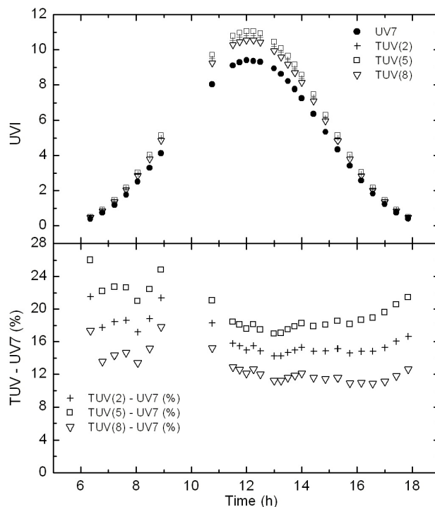
Fig. 14. Upper panel: UVI measurements and calculations for Melbourne (day 326) for modelling cases TUV(2,5,8) as a function of time. Lower panel: Relative model-measurement differences for the three modelling cases as a function of time.
