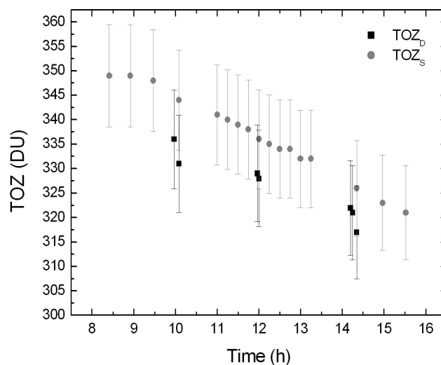
Fig. 7. Comparison between TOZ measurements with Dobson spectrophotometer and from the spectral measurements for day 63 of 2000 in Boulder. Error bars account for the \pm 3\% uncertainty from each source (as from Table 6).
