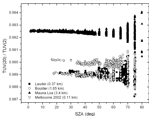
Fig. 6. Relative change in the calculated UVI caused by changing galb from 0.05 (TUV(2)) to 0.02 (TUV(20)) for the datasets in Fig. 1.
