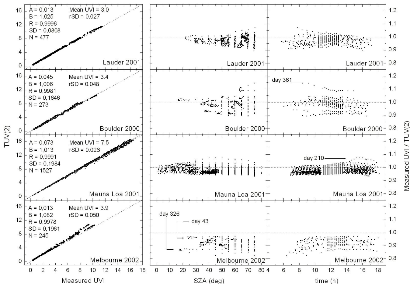
Fig. 9. Left panel: Regression plot of Modelled (TUV(2)) versus Measured UVI for four sites. Statistic parameters for regressions are shown. Right panel: Measured UVI/TUV(2) as a function of SZA and local time.
