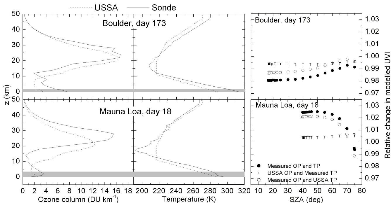
Fig. 5. Left panel: USSA profiles and measured OP and TP from 0 to 50 km for day 173 in Boulder and day 18 in Mauna Loa. Shaded regions show the parts of the profiles underneath the altitude level of each site. Right panel: Relative change in modelled UVI from considering measured OP and USSA TP (open circles), USSA OP and measured TP (T) and measured OP and TP (solid circles) in relation to case TUV(2) (USSA OP and TP).
