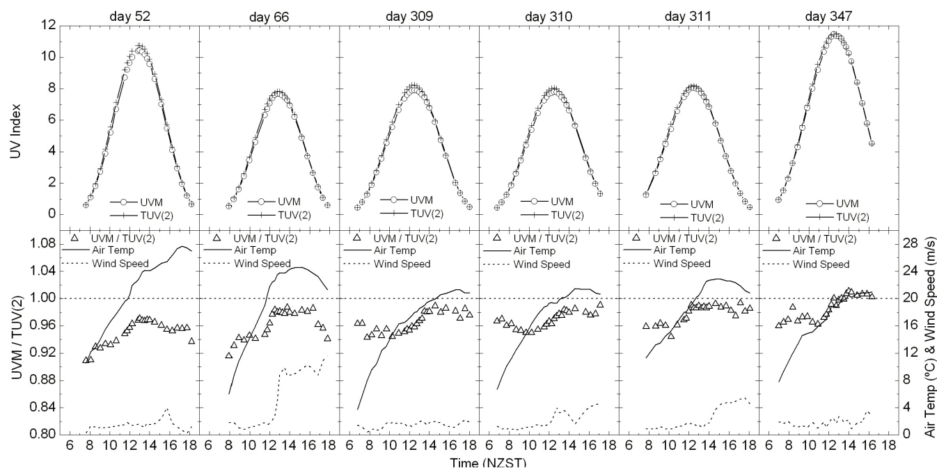
Fig. 11. UVI model vs. measurement comparison for six days of 2001 in Lauder for which air temperature clearly exceeded 20^{\circ}\text{C} and diurnal variations in TOZ and AOD were small. Upper: Measured (circles) and modelled (crosses) UVI as a function of time. Lower: Measured over modelled UVI ratio (triangles), air temperature (solid line) and wind speed (dashed line) as a function of time.
