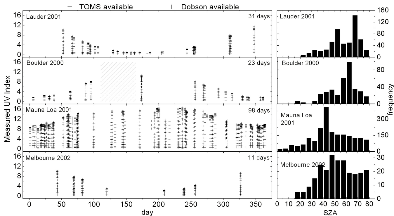
Fig. 1. Left panel: Clear-sky measured UVI for the four sites as a function of day, representing the considered datasets for this study. Availability of TOZ from TOMS and Dobson is shown through horizontal and vertical dashes, respectively. No UVI measurements were available from day 110 to 165 of 2000 in Boulder (hatched zone). Right Panel: Corresponding histogram of SZA.
