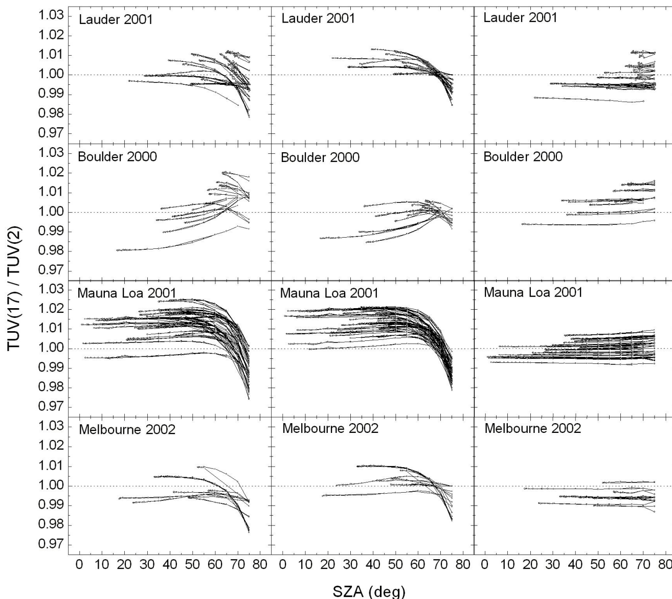
Fig. 4. Calculated effect on modelled UVI of using measured profiles of ozone and/or temperature, compared with using the USSA profiles for the datasets in Fig. 1. Plots are restricted to \text{SZA} \leq 75^\circ . Column 1: measured OPs and TPs are used. Column 2: measured OPs, but USSA TPs. Column 3: measured TPs, but USSA OPs.
