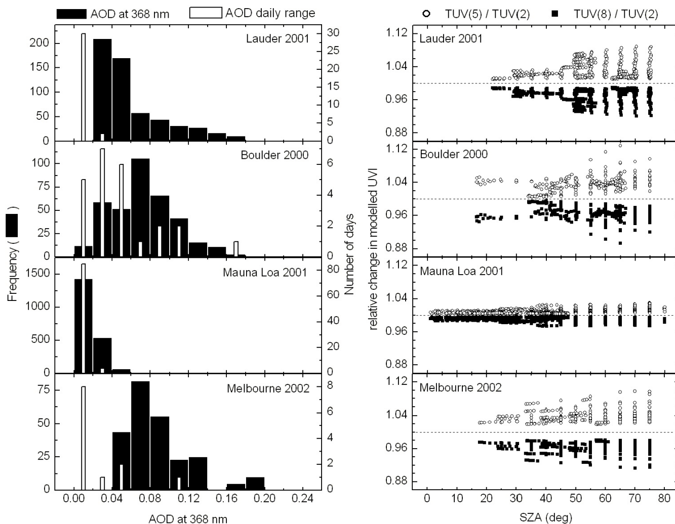
Fig. 3. Left panel: Histograms of AOD at 368 nm (in black) and its daily range (in white) for the datasets in Fig. 1. Right panel: TUV( i )/TUV(2), for i =5 (no aerosols, circles), and i =8 (SSA=0.7, squares).
