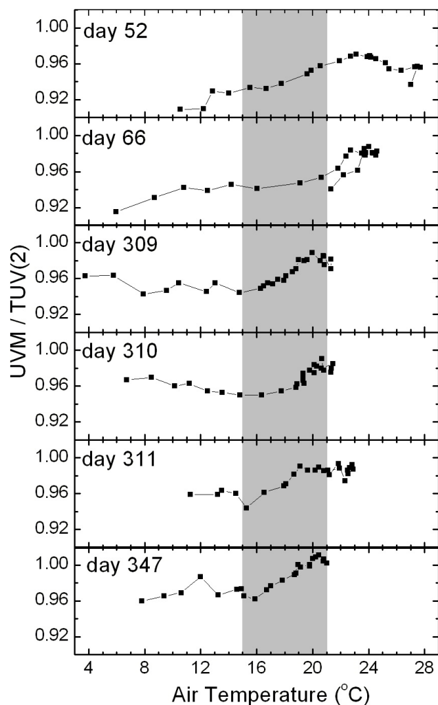
Fig. 12. From days represented in Fig. 10, measured over modelled UVI as a function of air temperature. The range of temperatures for which the PTFE temperature effect is expected to occur (15 to 21°C) is shaded.
