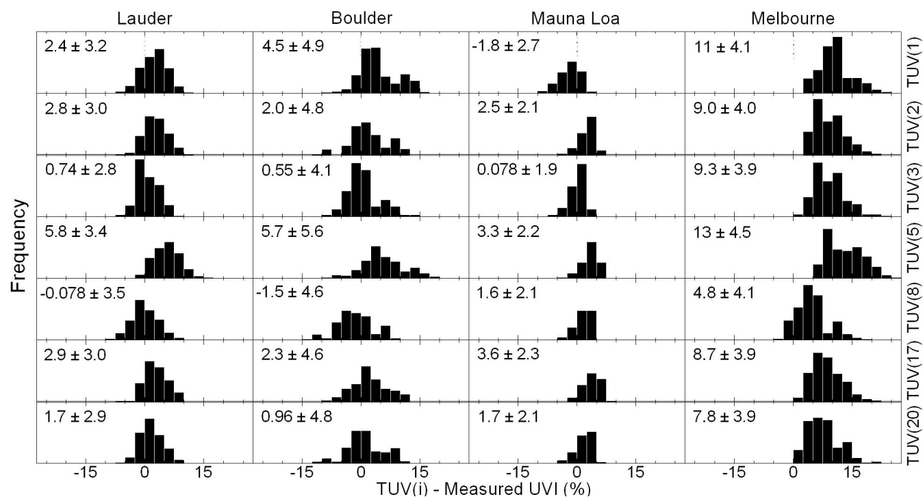
Fig. 8. Histograms of model-measurement relative differences for all sites and modelling cases TUV(1,2,3,5,8,17,20). Mean differences plus minus their standard deviations are shown for each case.
