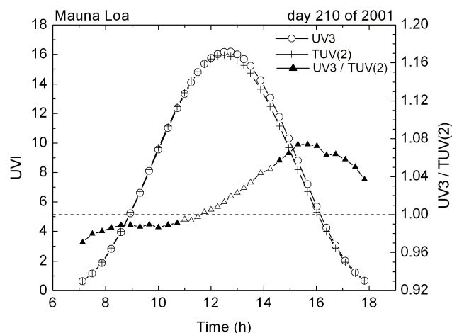
Fig. 13. Measured (circles) and modelled (crosses) UVI, and their ratio (triangles) for day 210 of 2001 in Mauna Loa. Open triangles account for data that was initially excluded from the study because AOD measurements were missing. Modelling for this period has been done using an AOD of 0.011 (AOD for that day ranged from 0.010 to 0.013) so to have an estimation of the increase in UVI measurements that happened around noon.
