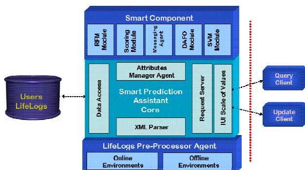
Fig. 3. Architecture of Smart Prediction Assistant.
