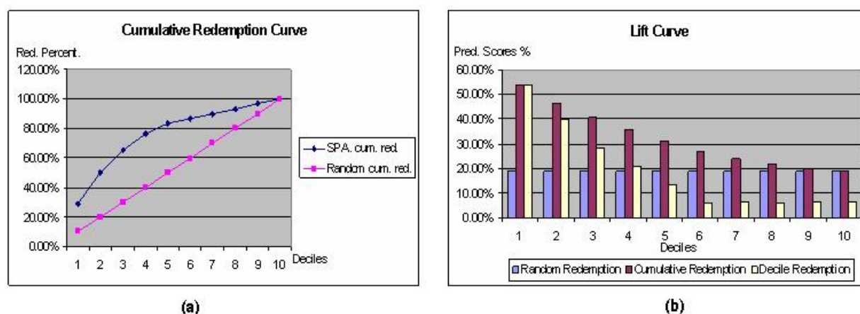
Fig. 6. Cumulative redemption curve (a) and Predictive Scores (b) for the increase in transactions of 1,340,432 users of emagister.com
