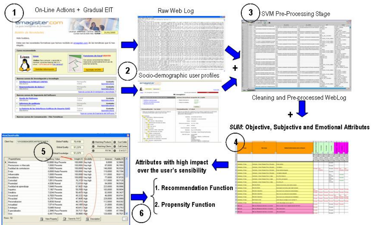
Fig. 4. Iterative automatic process to discover, manage and update emotional attributes in SPA.
