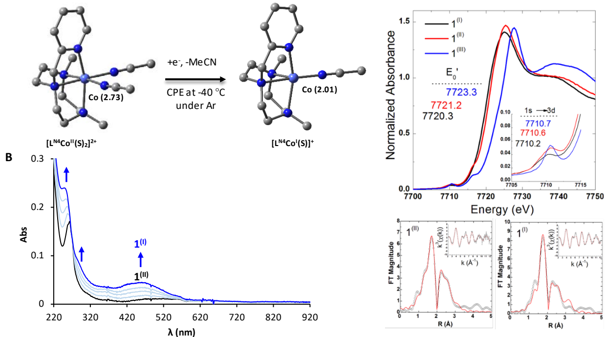
Figure 3. A) DFT (B3LYP-D 3 /6-31+G*) modeled structures for the most stable Co II ([L N4 Co II (CH 3 CN) 2 ] 2+ ) and Co I ([L N4 Co I (CH 3 CN)] + ) species under the reaction conditions. The spin density over cobalt center is shown in parentheses. B) UV-Vis-SEC of 1 (II) (black trace) at -1.7 V to yield a new reduced species (blue trace). C) Co K-edge XANES of complex 1 in I, II and III oxidation states with inset showing the pre-edge area of the 1s → 3d transitions. D) Fourier transformed EXAFS data and fits with the inset showing the k-space spectra (Data (circles) Fit (red)).
