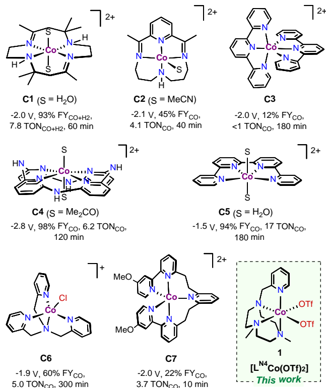
Chart 1. Selected cobalt catalysts for electrochemical CO 2 -to-CO reduction. 5c,8,9b,c,14-15 See Table S1 for further details.
