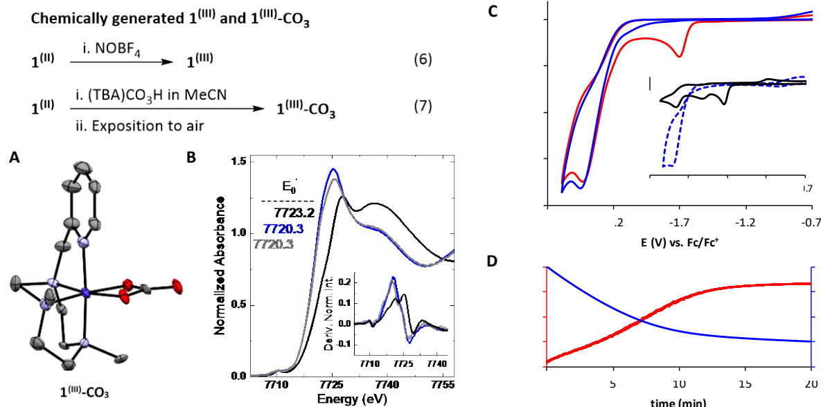
Figure 4. Chemical equations for the generation of 1^{(III)} and 1^{(III)}\text{-CO}_3 . A) ORTEP plot of the 1^{(III)}\text{-CO}_3 X-ray crystal structure (see SI for structural parameters). B) Co K-edge XANES of the solution after CPE at -1.7 V (blue), the chemically generated references of 1^{(II)}\text{-CO}_3 (grey) and 1^{(III)}\text{-CO}_3 (black) with inset showing each first derivative. C) CVs of 1^{(III)} (1 mM) under \text{CO}_2 before (red) and after (red dashed) electrolysis at ca. -1.9 V. Inset: CVs under Ar (black) and under \text{CO}_2 in the presence of 1 eq. of \text{TBACO}_3\text{H} (blue dashed). D) Current and charge profiles along electrolysis of 1^{(III)} (1 mM) under \text{CO}_2 . Electrolysis and CVs ( 0.1 \text{ V}\cdot\text{s}^{-1} ) recorded in anhydrous \text{TBAPF}_6/\text{CH}_3\text{CN} (0.1 M) over carbon mesh and glassy carbon, respectively.
