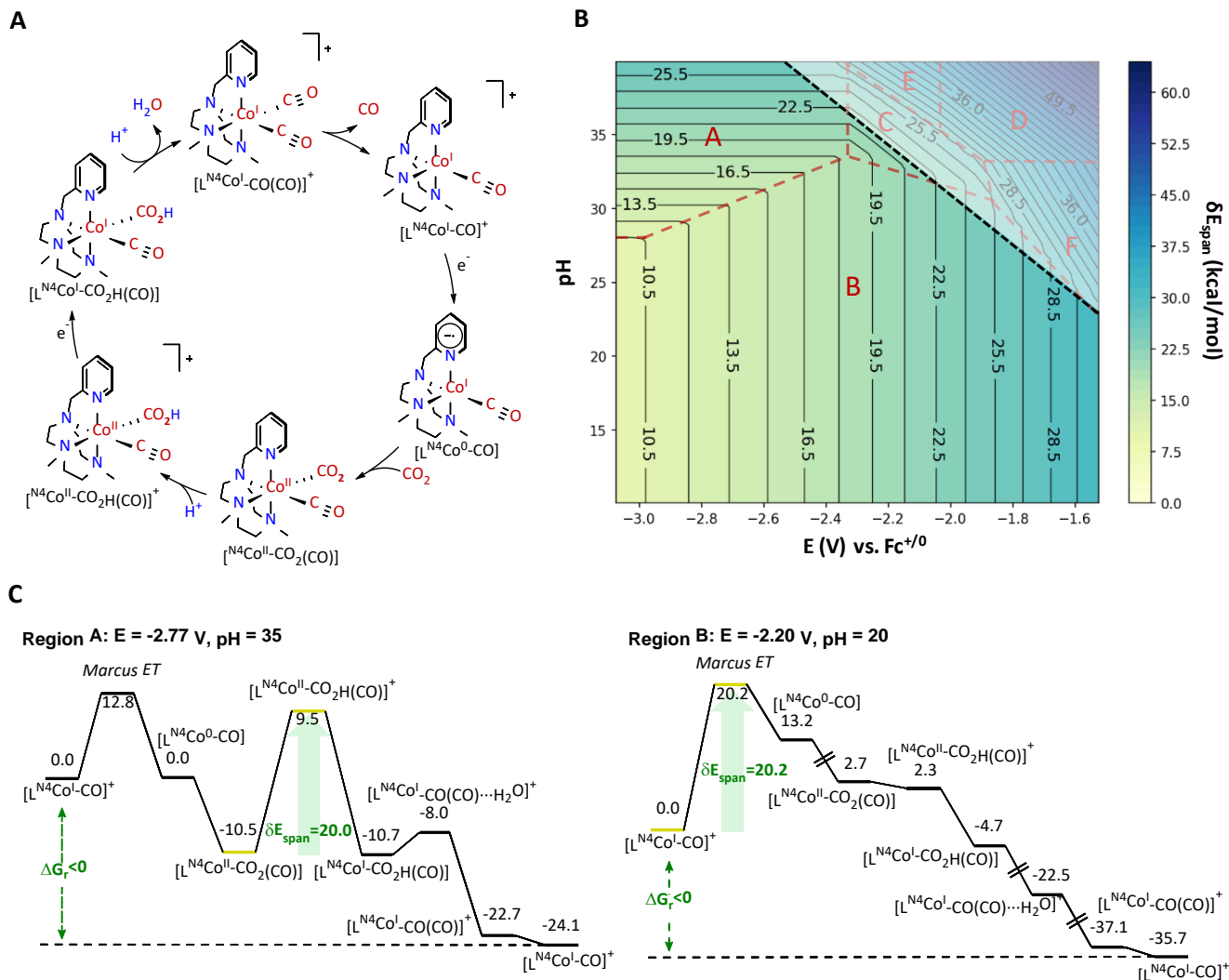
Figure 7. A) Proposed reaction mechanism for the CO 2 reduction to CO catalyzed by 1 0 -CO. B) Contour-plots of the kinetic energy span \delta E_{\text{span}} (color scale, kcal·mol -1 ) of the calculated reaction mechanism versus the applied reduction potential (horizontal axis, V vs. Fc/Fc + ) and the pH (vertical axis). Regions A-F are delimited by dashed red lines and the dashed black line spares the thermodynamic ( \Delta G_r < 0 kcal·mol -1 ) regime from the non-thermodynamic one ( \Delta G_r > 0 kcal·mol -1 ). C) Gibbs energy profiles associated with Regions A and B.
