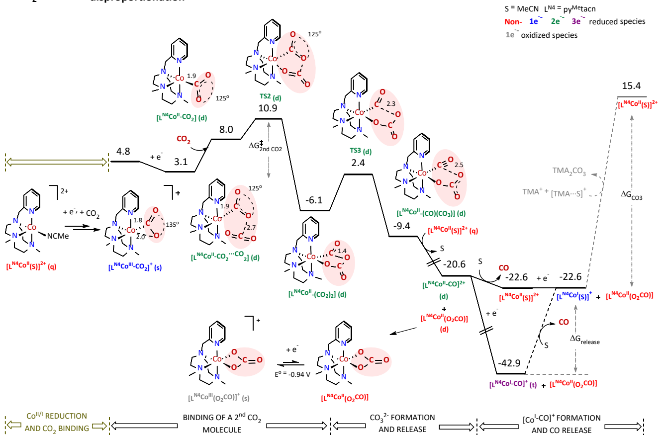
Figure 5. Computed Gibbs energy profile for the [L^{N4}Co^I-CO]^+ formation through the CO_2 reduction to CO mediated by 1^{(II)} at a working potential of -1.91 V vs. Fc/Fc^+ and pH 25. Energies and other relevant thermodynamic and structural parameters are given in kcal \cdot mol^{-1} , V vs. Fc/Fc^+ , Å and degrees. The spin multiplicity of each intermediate is shown in parenthesis: singlet (s), doublet (d), triplet (t), quartet (q). TMA = tetramethylammonium.
