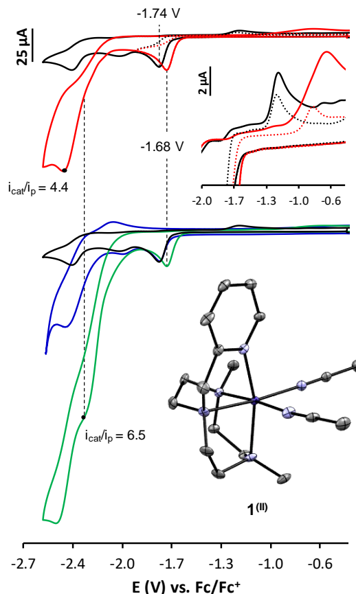
Figure 1. CVs of 1 III (1 mM) in anhydrous TBAPF 6 /CH 3 CN (0.1 M) solution at \nu = 0.1 \text{ V} \cdot \text{s}^{-1} . Top ) under Ar (black) and CO 2 (red); Inset: magnification range between -2.0 to -0.5 V. Scans window from -0.5 to -1.9 V are shown with dotted lines. Bottom ) under Ar (black), and with added H 2 O (0.55 M) under Ar (blue) and CO 2 (green). Inset: X-ray crystal structure of complex 1 III , triflate counterions and hydrogen atoms have been omitted for clarity.
