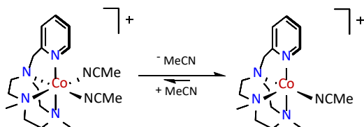
Scheme 3. Proposed penta/hexa coordination equilibrium of the electrochemically generated cobalt(I) species.
