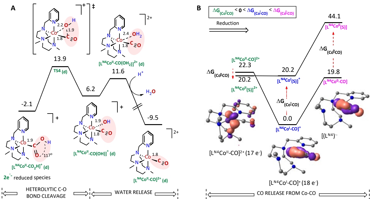
Figure 6. A) Heterolytic C-O bond cleavage step starting from [\text{L}^{\text{N}4}\text{Co}^{\text{II}}\text{-CO}_2\text{H}]^+ to form [\text{L}^{\text{N}4}\text{Co}^{\text{II}}(\text{CO})(\text{OH})]^+ intermediate. B) Thermodynamics of the \text{Co}^{\text{II}/\text{I}/0} one electron reductions and each corresponding CO release step. Selected singly occupied molecular orbital of \text{Co}^{\text{II}/\text{I}/0} -CO complexes (isovalue 0.07). Energy profiles computed at -1.91 V vs. \text{Fc}/\text{Fc}^+ and pH 25.
