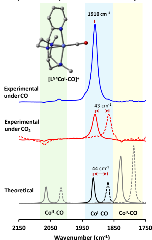
Figure 2. Top and middle: Experimental spectra obtained by FTIR-SEC of a 0.2 M TBAPF 6 /CH 3 CN solution of 1 (6 mM) under CO (blue) and CO 2 (red) at ca. -1.7 V ( 12 CO 2 plane, 13 CO 2 dashed). Bottom: Theoretical v CO bands of 1 (II) -CO, 1 (I) -CO and 1 (0) -CO ( 12 CO 2 red line, 13 CO 2 dashed line) calculated at the B3LYP-D 3 (SMD)/6-31+G* level of theory.
