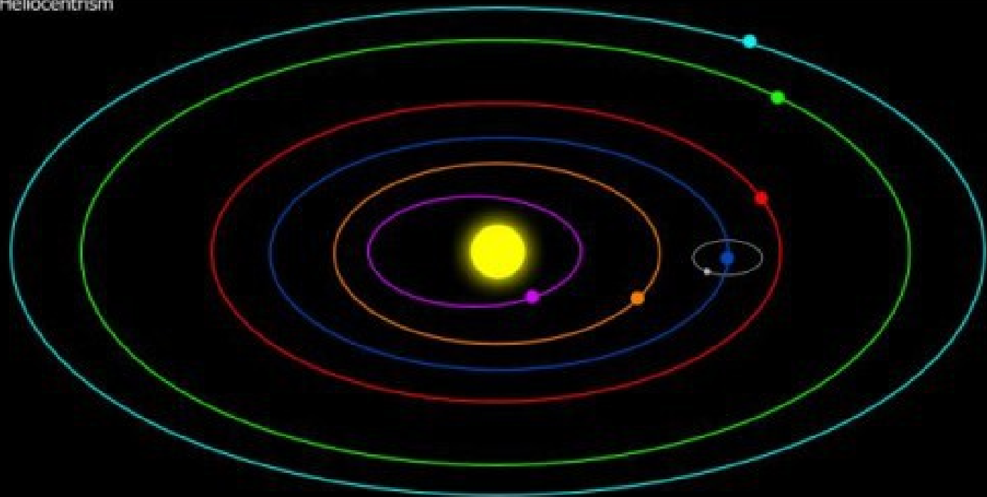
Heliocentrism
