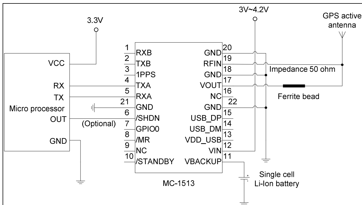
Fig 3-3 Typical application circuit that uses active antenna. (UART communication)
