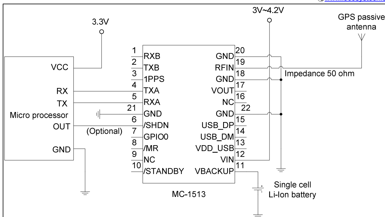
Fig 3-2 Typical application circuit that uses passive antenna. (UART communication)
