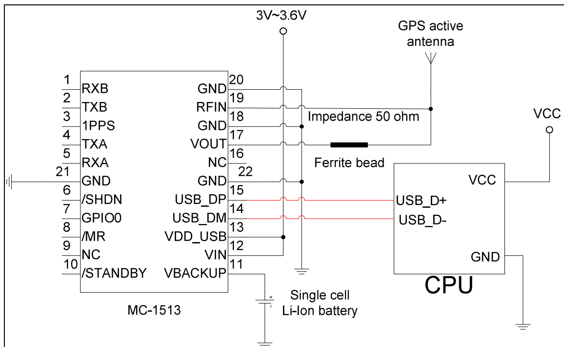
Fig 3-5 Typical application circuit that uses active antenna. (USB communication)
