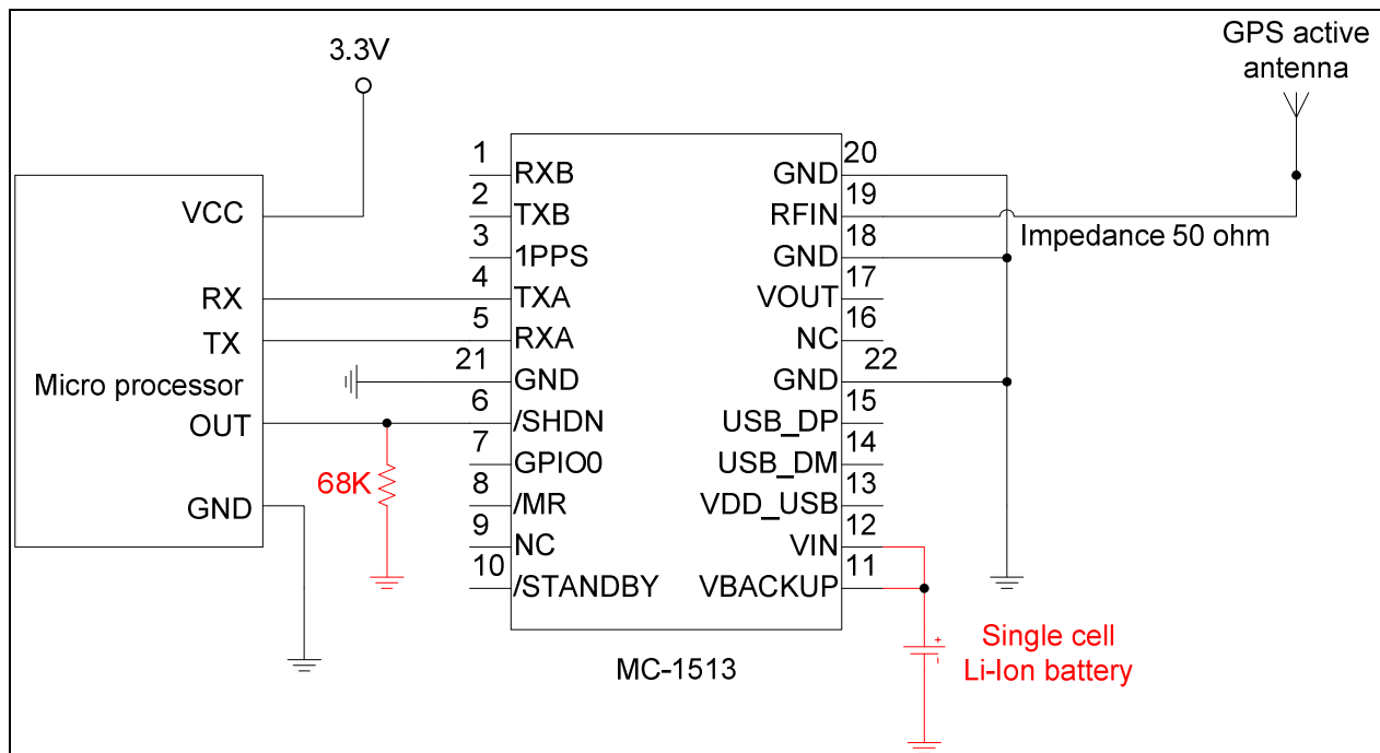
Fig 3-4 Typical application circuit that directly uses a Li-Ion battery as power source.
