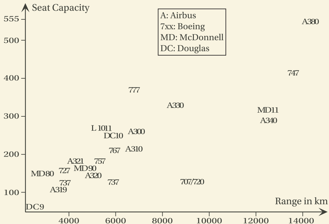
Figure 11.5: Aircraft Characteristics along Size and Range
