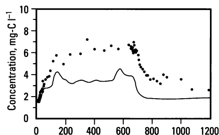
Figure 7. Observed (●) and simulated (—) NOM breakthrough curves at the withdrawal well.
